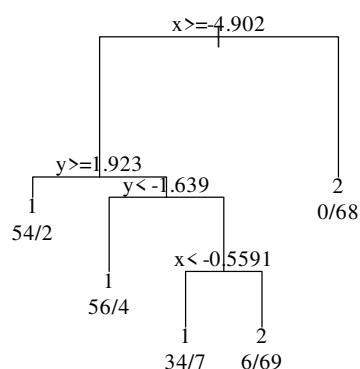
Figure 13.11: The optimal tree for the bivariate test data. This tree misclassifies 19 of the 300 samples in the training data (6.3%). The 10-fold cross validation error is 18%.
