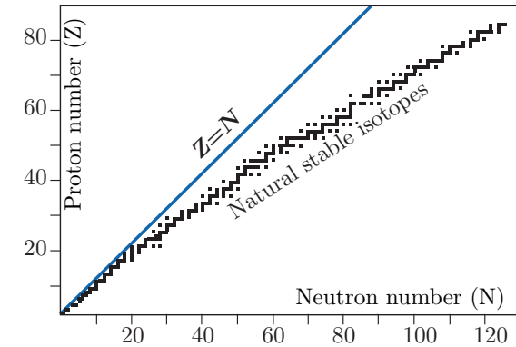
Figure 2.1: A schematic ‘Chart of Nuclides’ (modified from Allègre, 2008).
