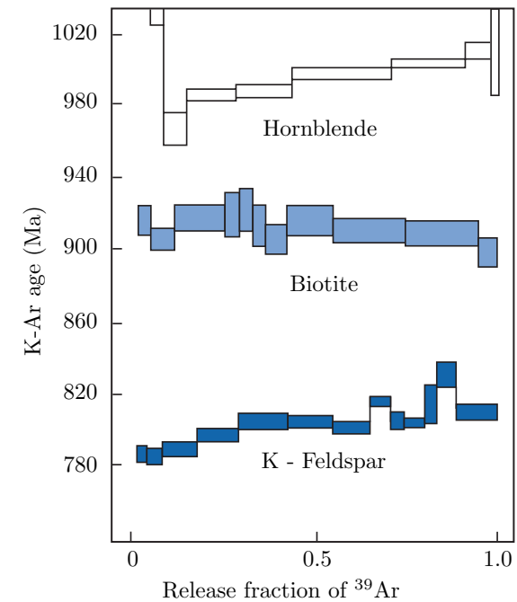
Figure 6.1: ^{40}\text{Ar}/^{39}\text{Ar} age spectra obtained by stepwise heating of three different K-bearing minerals. Biotite exhibits a flat ‘plateau’, indicating a simple history of rapid crystallisation and/or cooling. K-feldspar shows a rising age spectrum, consistent with a more complex evolution comprising multiple growth phases and/or thermal resetting. Finally, hornblende shows a ‘U-shaped’ release spectrum in which the first heating step releases a large amount of ‘excess’ argon (modified from Allègre, 2008).
