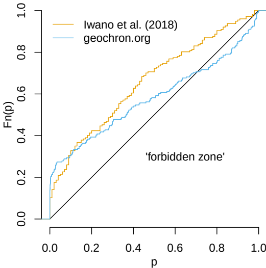
Figure 7. The yellow curve represents a fission track dataset of reference materials (Iwano et al., 2018), which shows no detectable evidence for cherry picking. In contrast, the blue curve corresponds to a compilation of fission track data in which 30% of the p-values are underdispersed to such a degree that they are ‘too good to be true’.
