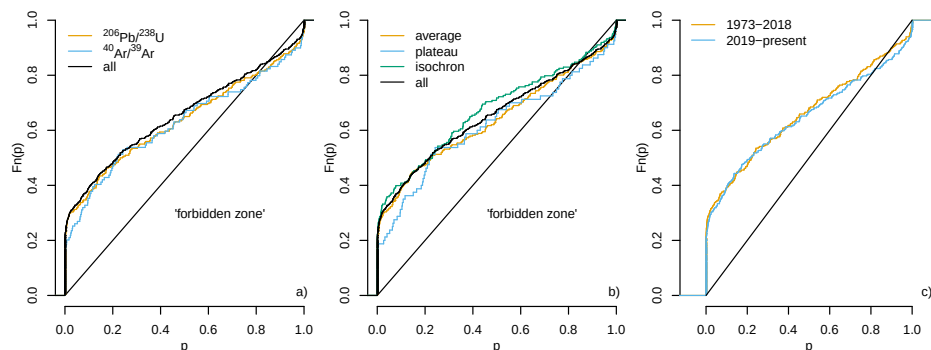
Figure 8. p-value distributions for the compilation of 100 Nature papers. The black curves represent the full dataset of 650 p-values. The colours group the dataset according to the geochronometer (a), plotting device (b) and publication year (c).
