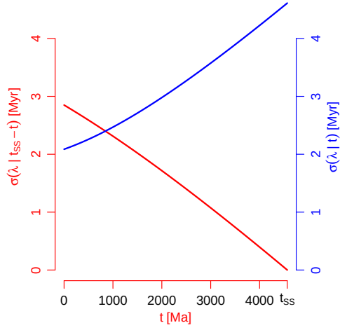
Figure 1: Decay constant uncertainty as a function of the ^{207}\text{Pb}/^{206}\text{Pb} age t (blue); and the difference between a meteorite of age t and the start of the solar system t_{SS} (red).
