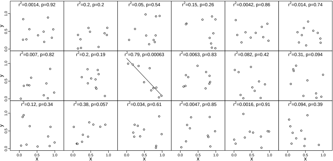
Figure A1. 18 scatter plots of bivariate random uniform data, with indication of the coefficient of determination ( r^2 ) and the p-value for correlation. The one ‘significant’ result (p-value = 0.00063) is a Type I error.
