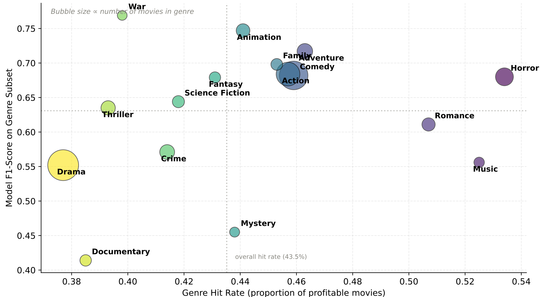
Figure 4.1 — Genre-Specific Hit Rate vs Model Predictability
