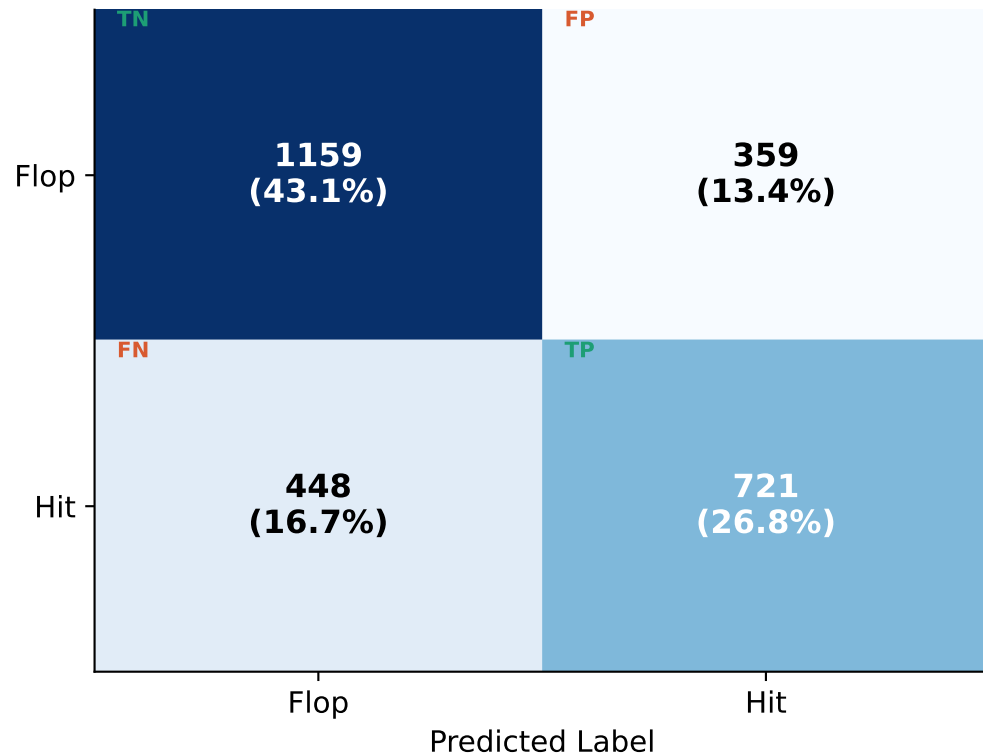
(a) Confusion matrix on test set
