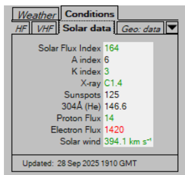
Figure 1.129 Solar Data
