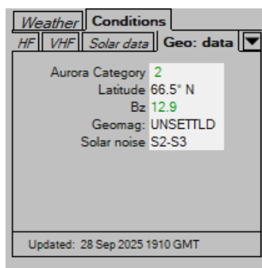
Figure 1.130 Geomagnetic Data
