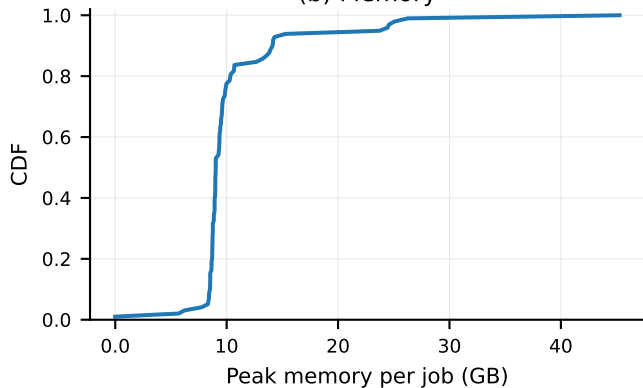
(b) Memory
