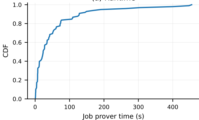
(a) Runtime
