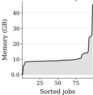
Peak memory
