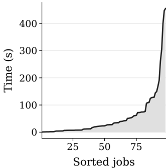
Prover time
