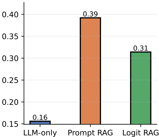
Exact Match (EM)
