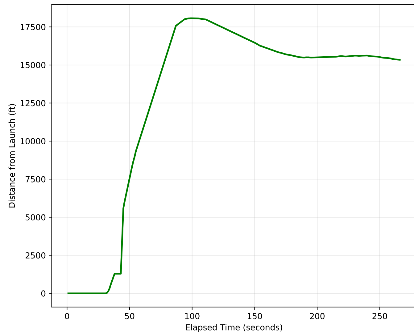
Filtered Horizontal Drift from Launch Point
