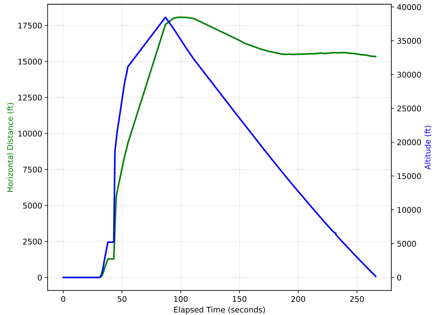
Altitude vs Filtered Horizontal Drift
