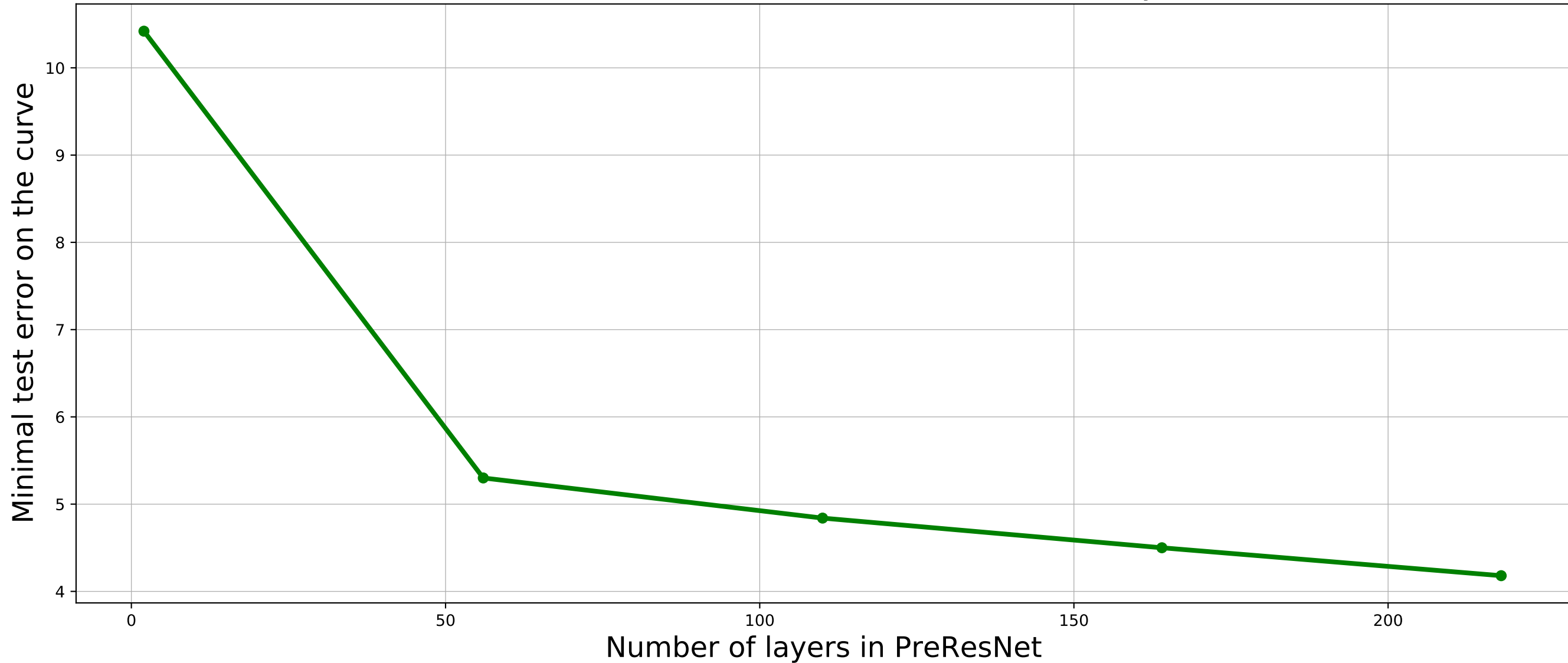
Minimal test error on the found Bezier curve to the number of layers in the network
