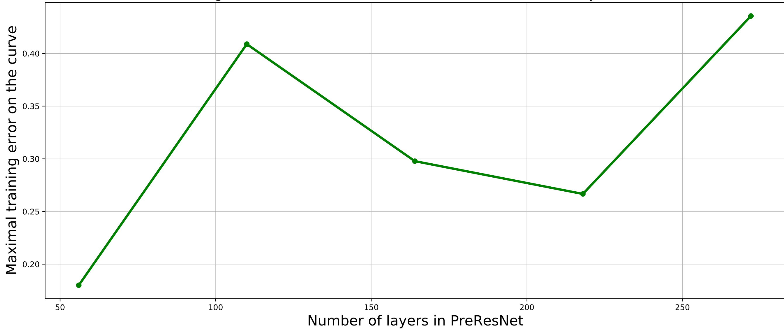
Maximal training error on the found Bezier curve to the number of layers in the network
