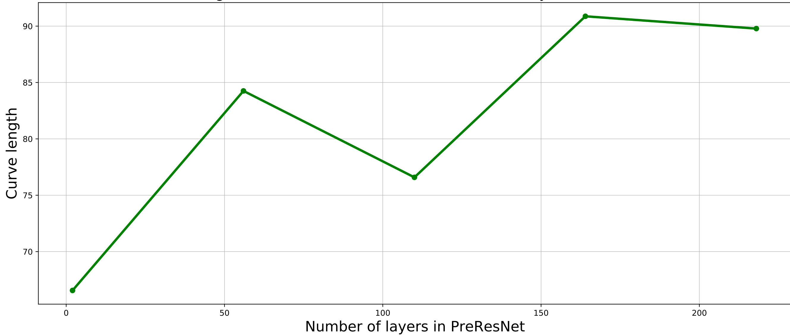
Total length of found Bezier curve to the number of layers in the network
