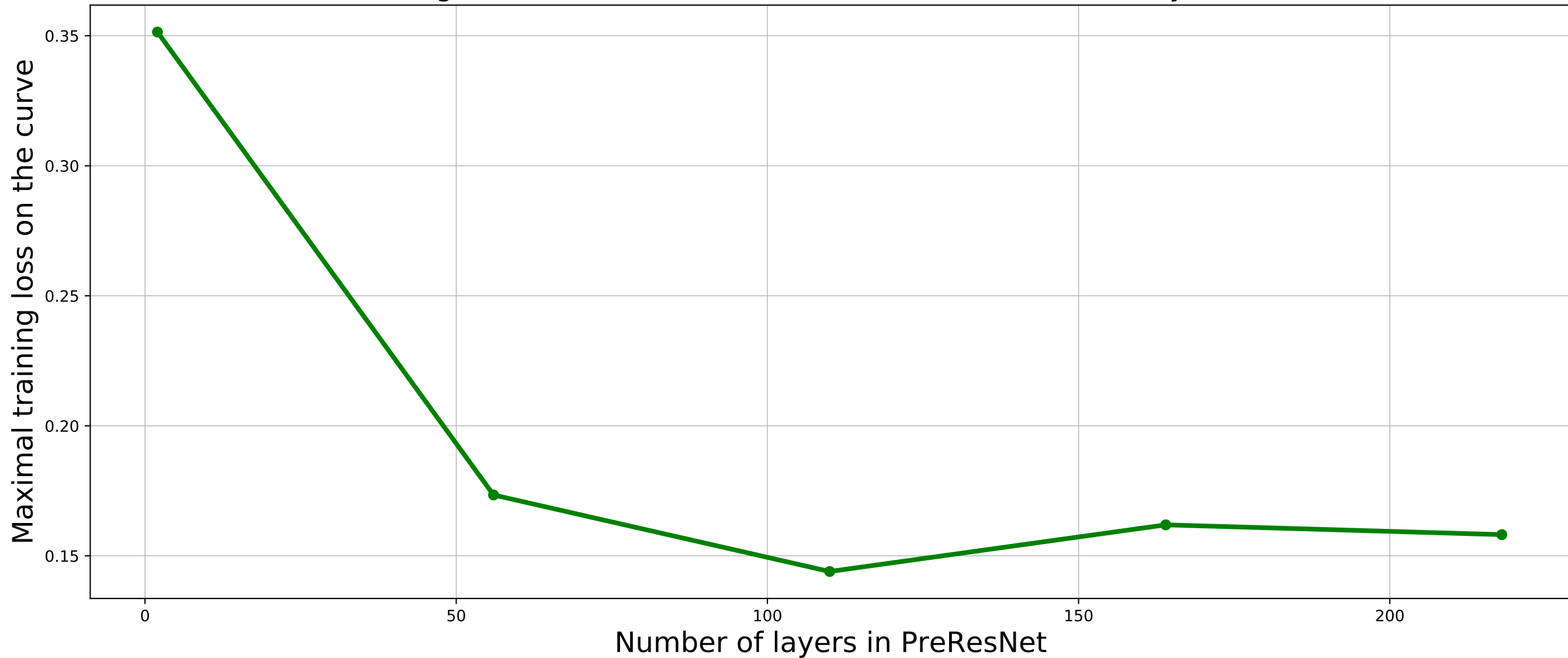
Maximal training loss on the found Bezier curve to the number of layers in the network
