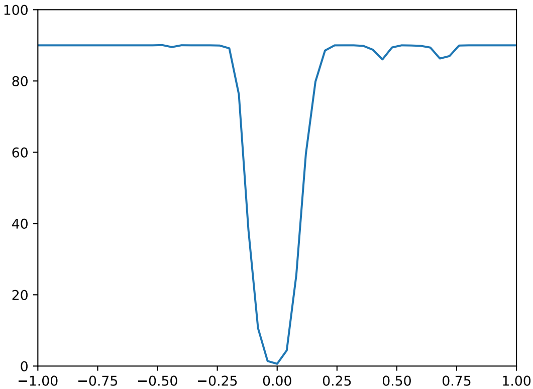
Training Error
