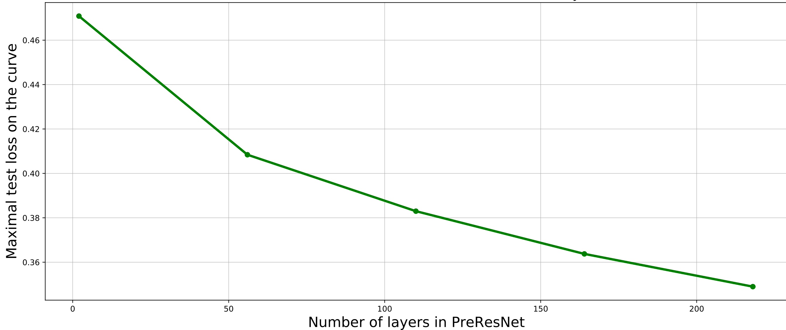
Maximal test loss on the found Bezier curve to the number of layers in the network
