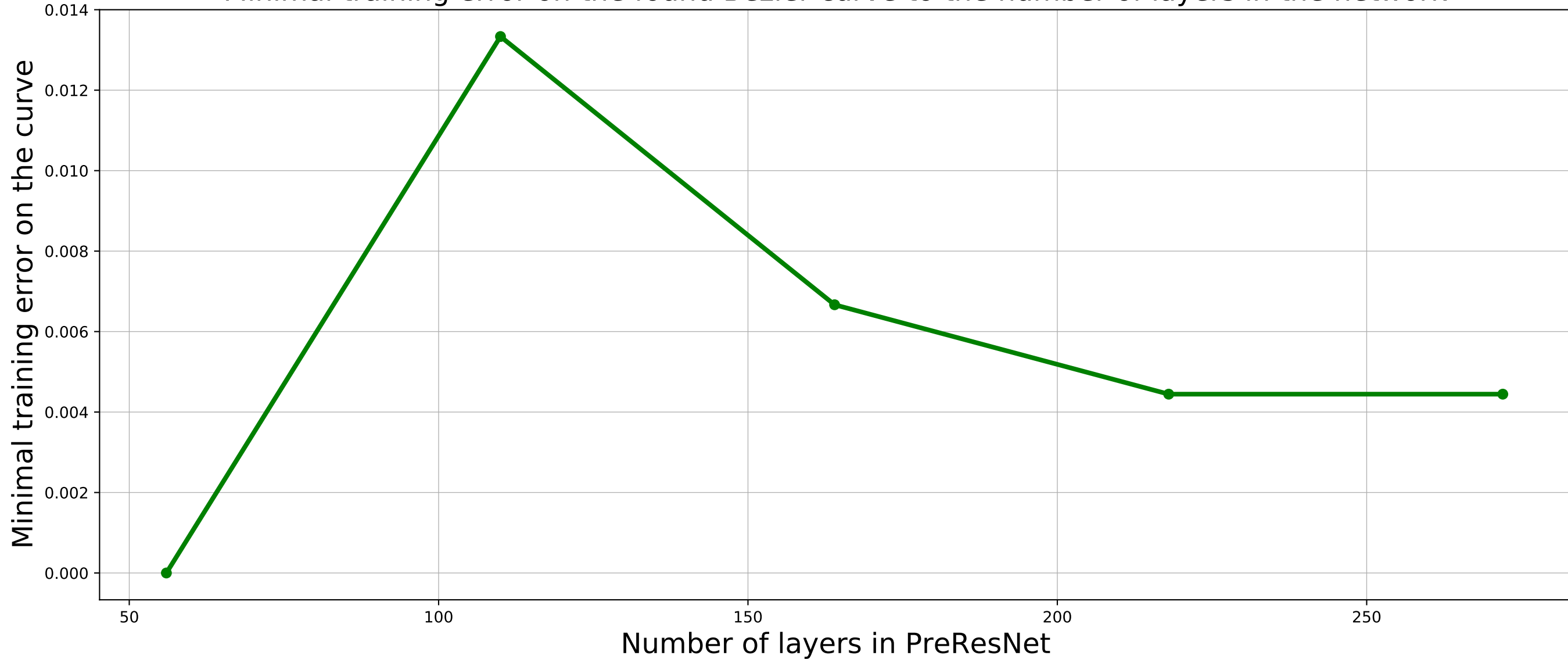
Minimal training error on the found Bezier curve to the number of layers in the network
