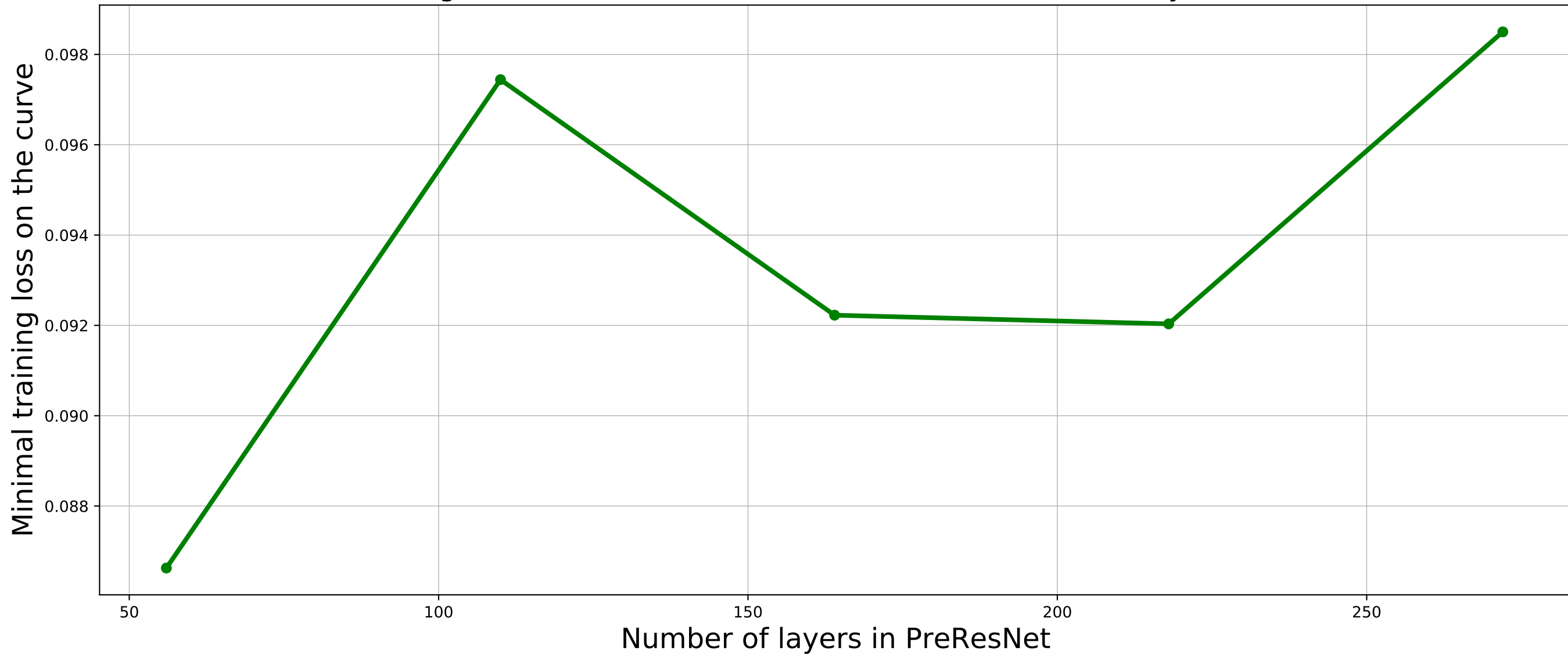
Minimal training loss on the found Bezier curve to the number of layers in the network
