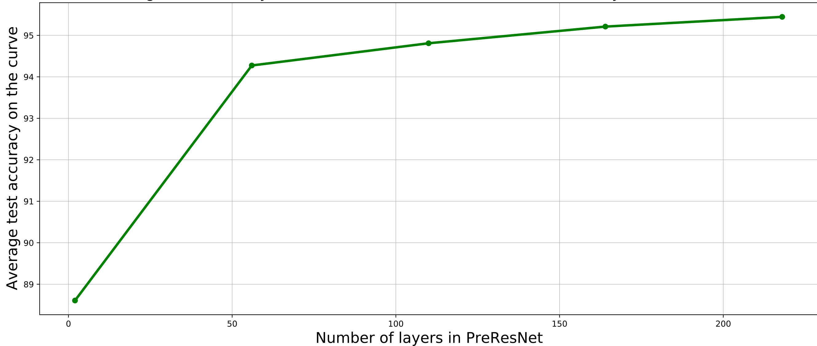
Average test accuracy on the found Bezier curve to the number of layers in the network
