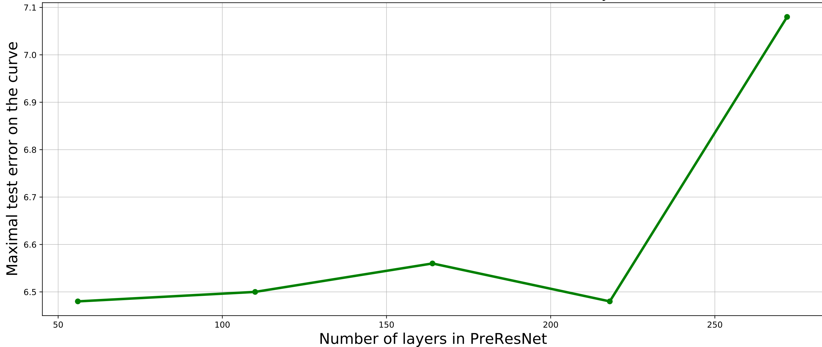
Maximal test error on the found Bezier curve to the number of layers in the network
