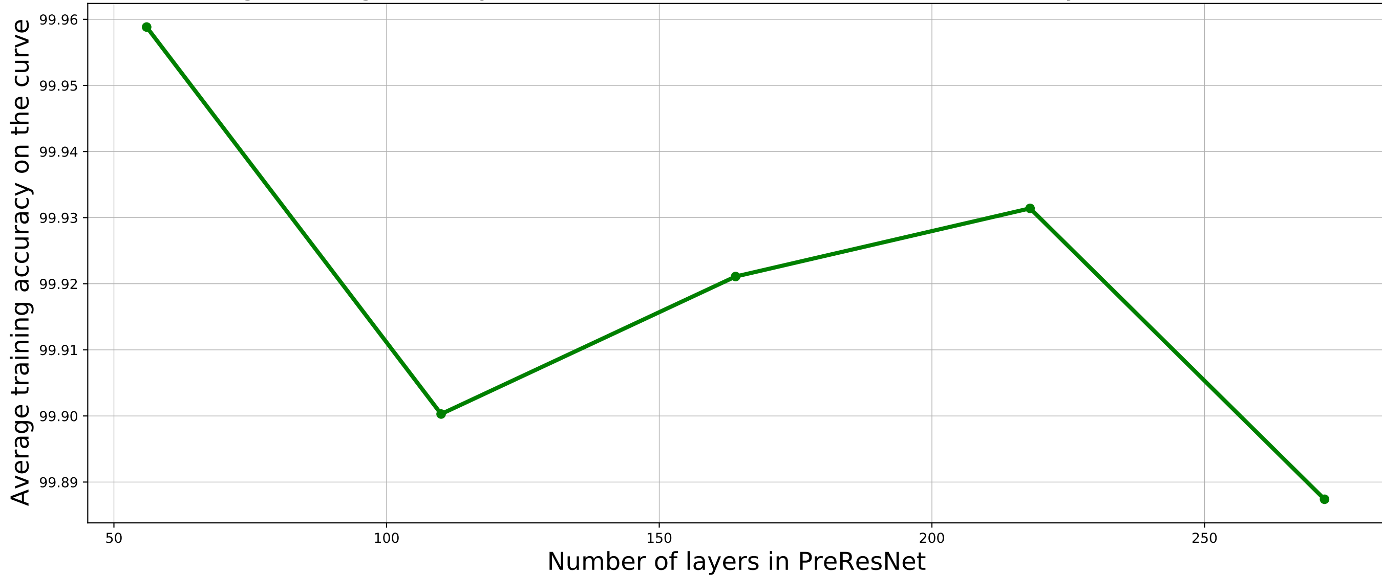
Average training accuracy on the found Bezier curve to the number of layers in the network
