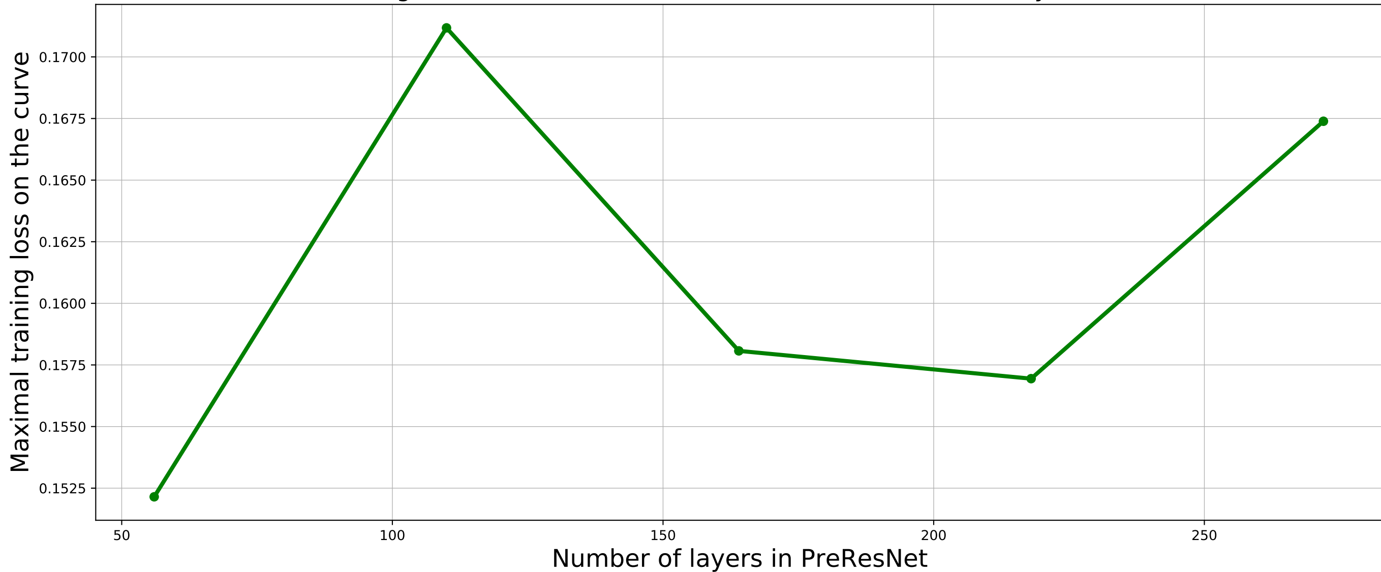
Maximal training loss on the found Bezier curve to the number of layers in the network
