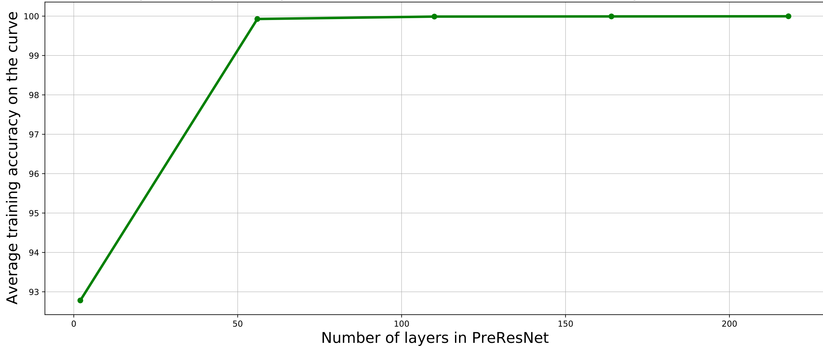
Average training accuracy on the found Bezier curve to the number of layers in the network
