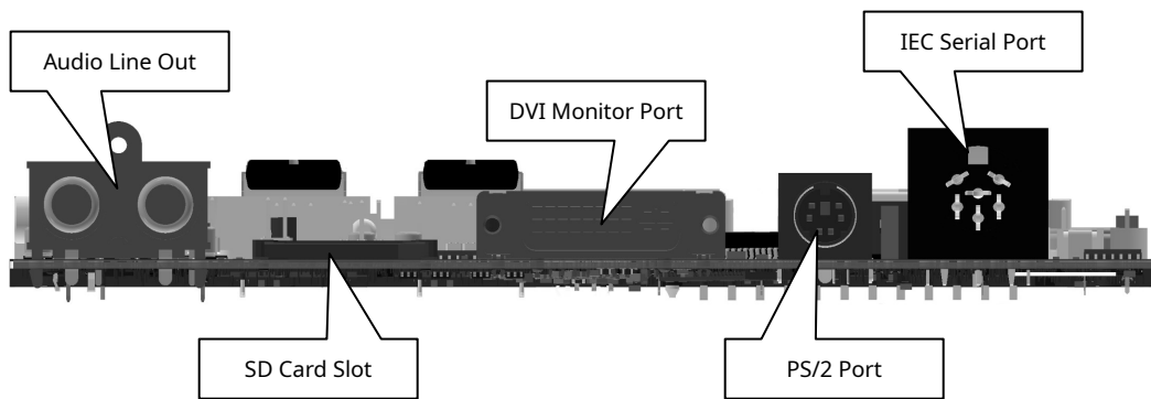
Figure 1.1: F256jr Rear Connectors
