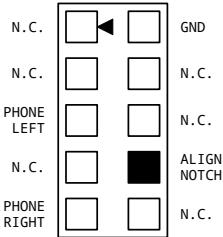
Figure 22.6: Case Audio Pinouts
