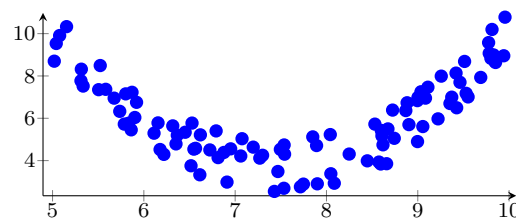
Quadratic/nonlinear shape
