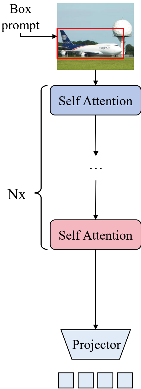
(a) Vision Encoders
