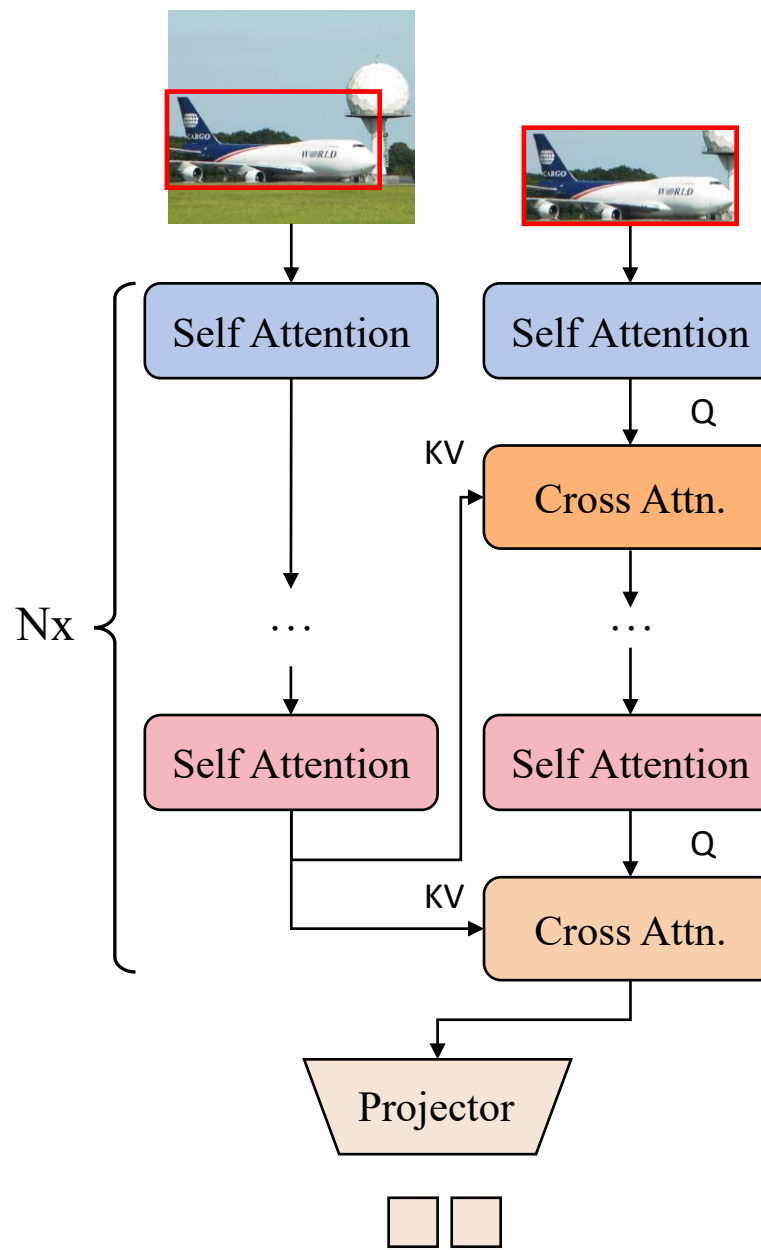
(c) Describe Anything
