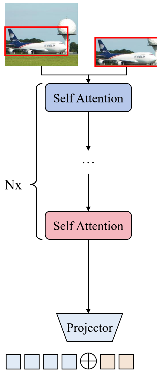
(b) Visual Perception Tokens
