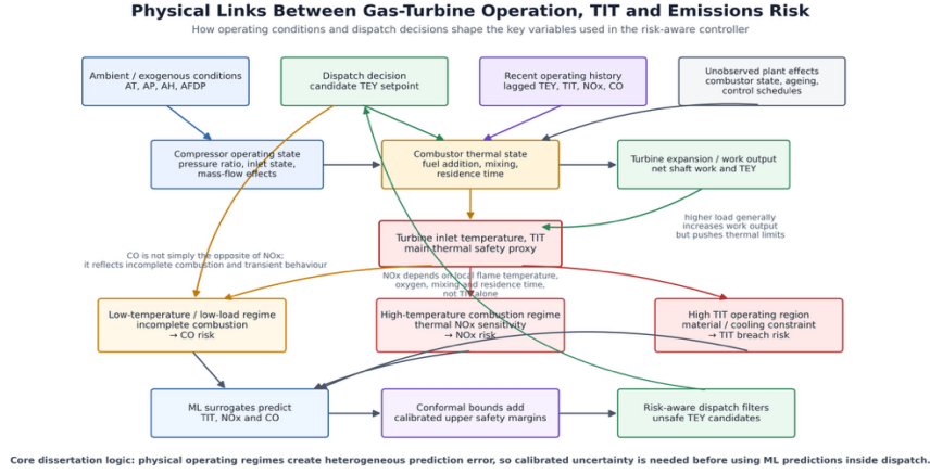
Figure 1: Figure 2 - Physical Links between Gas Turbine operation, TIT, and Emissions risk
