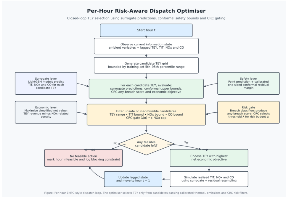
Figure 3: Figure 4 - Per hour dispatch optimiser
