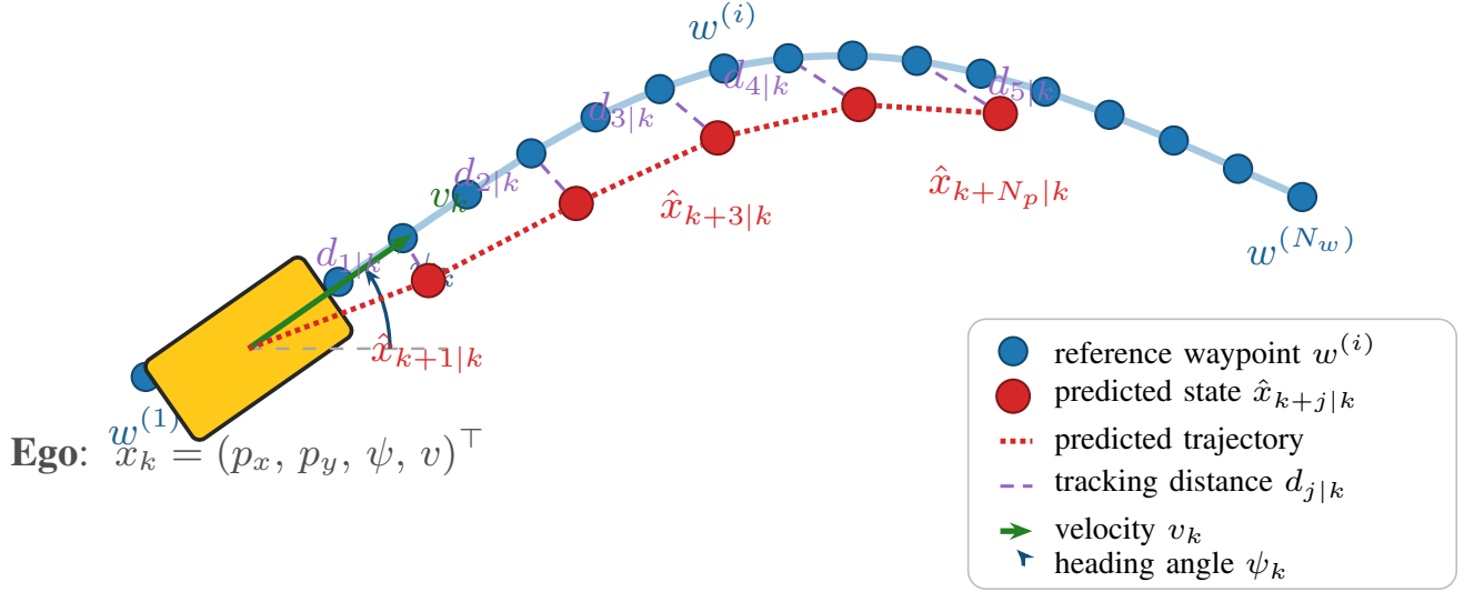
Fig. 1. MPC waypoint-tracking formulation. The ego vehicle at position (p_x, p_y) moves with speed v_k and heading \psi_k (measured from east, shown as an arc). Reference waypoints \{w^{(i)}\}_{i=1}^{N_w} (blue) define the desired path. At each step k , MPC rolls out the kinematic bicycle model (11) to obtain N_p predicted states \hat{x}_{k+j|k} (red) and minimizes the sum of squared distances d_{j|k} (purple dashed) from each predicted position to the closest waypoint (13).
