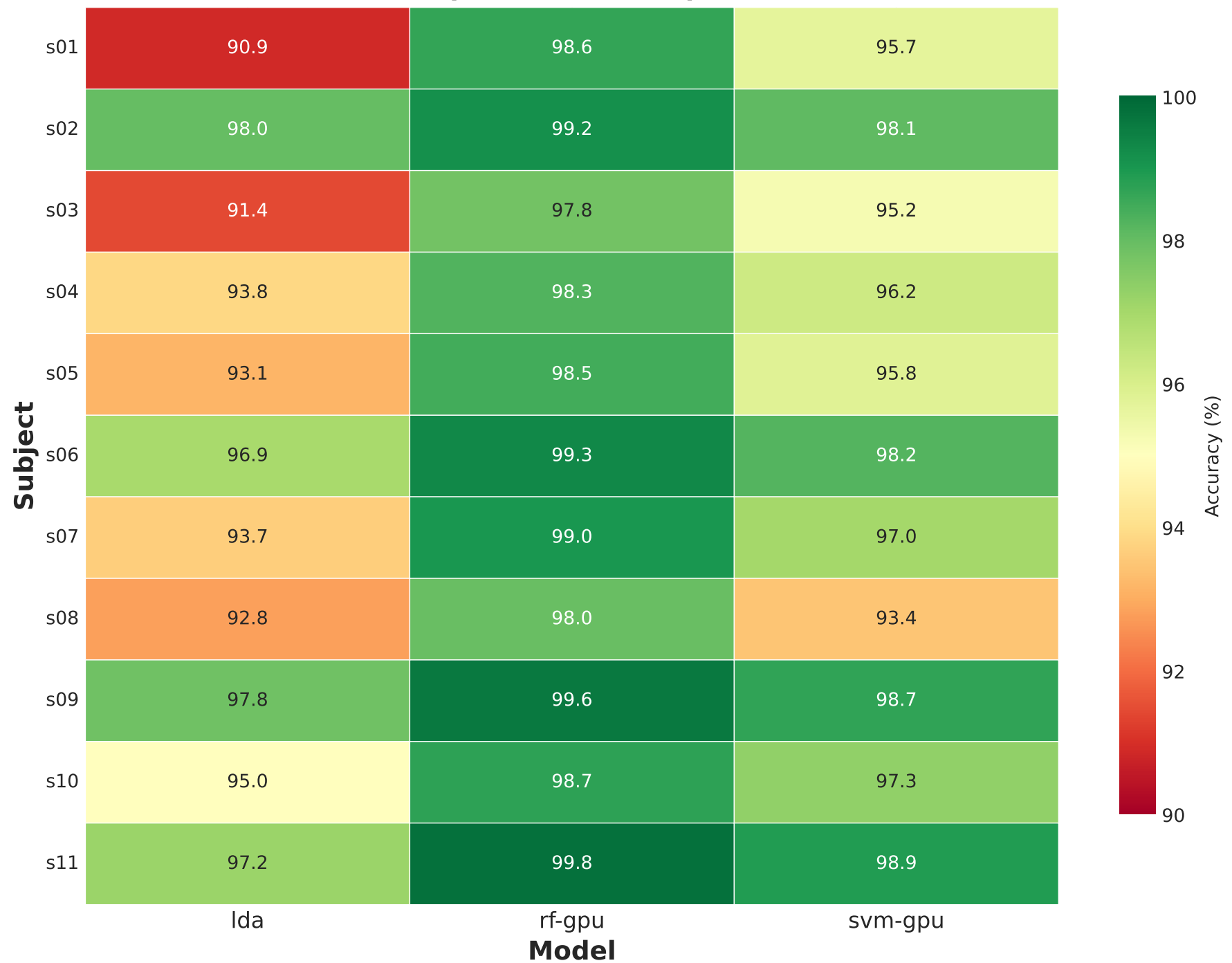
Within-Subject CV Accuracy (%) by Subject and Model (RAMI Dataset)
