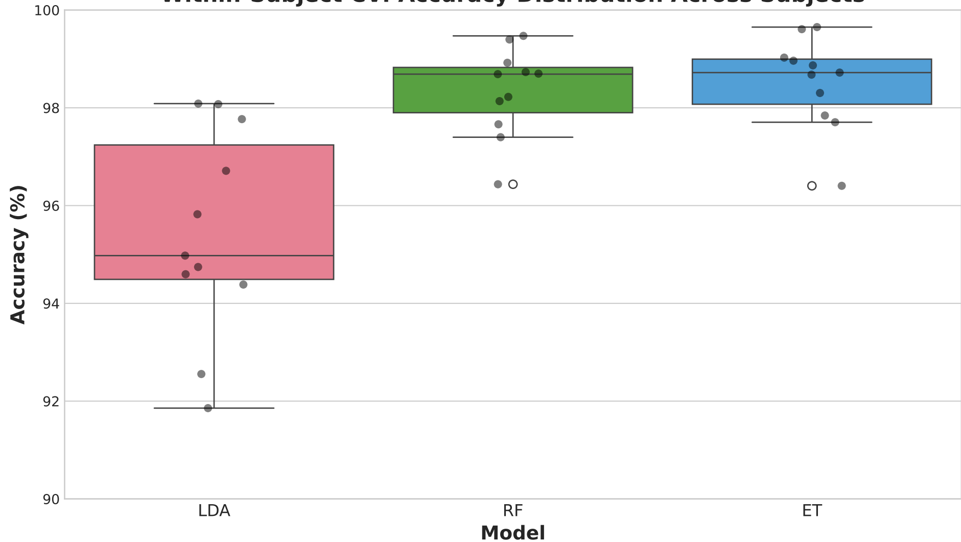
Within-Subject CV: Accuracy Distribution Across Subjects
