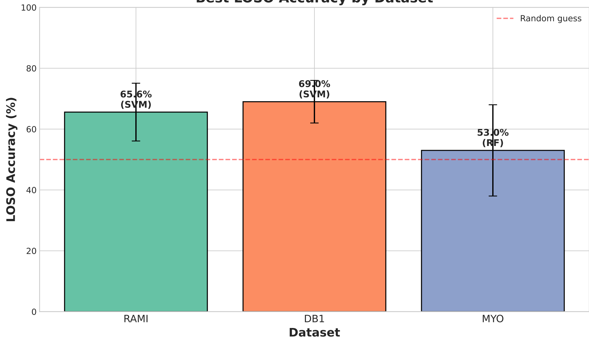
Generalization Gap Across Datasets
