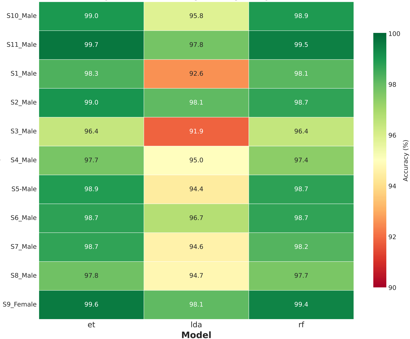
Within-Subject CV Accuracy (%) by Subject and Model
