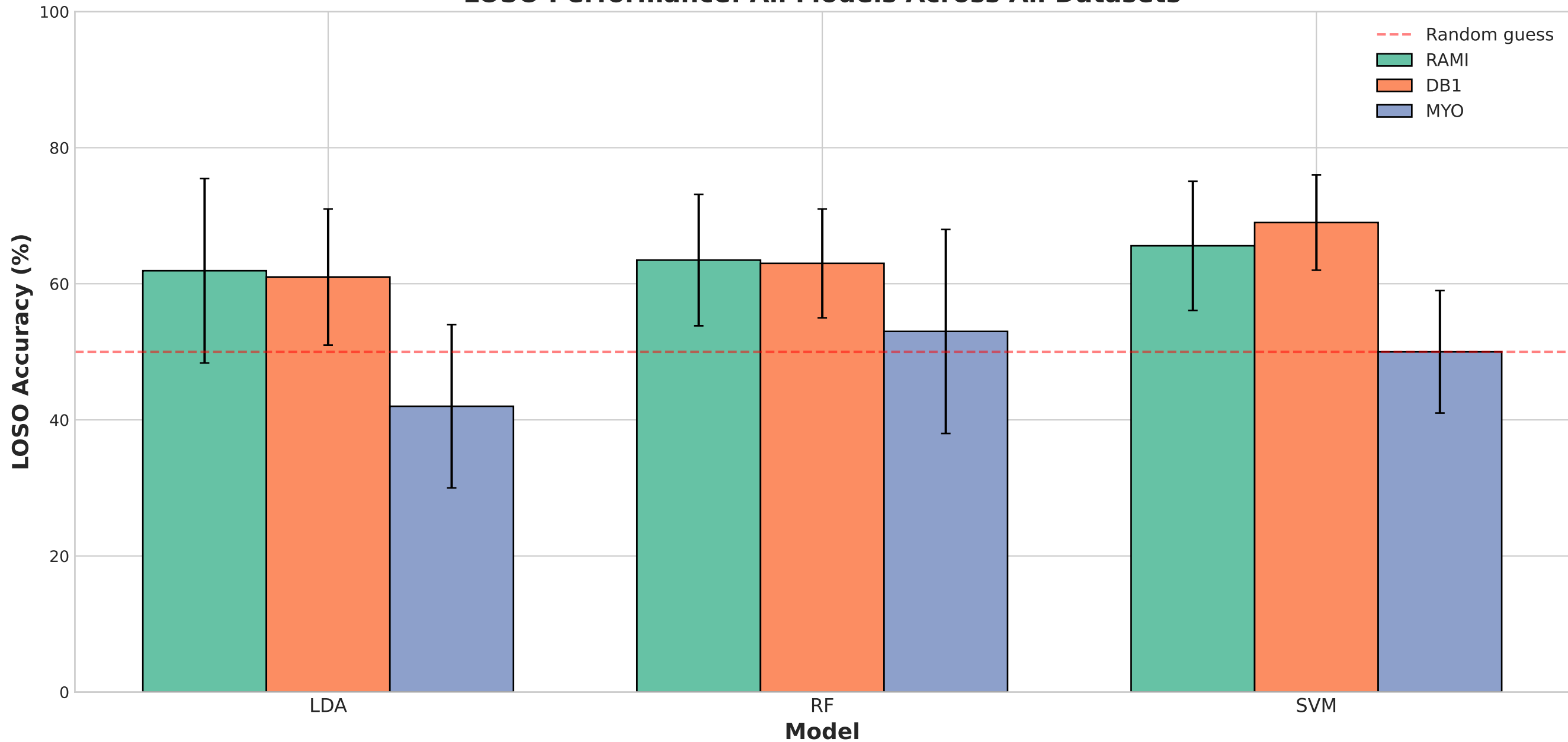
LOSO Performance: All Models Across All Datasets
