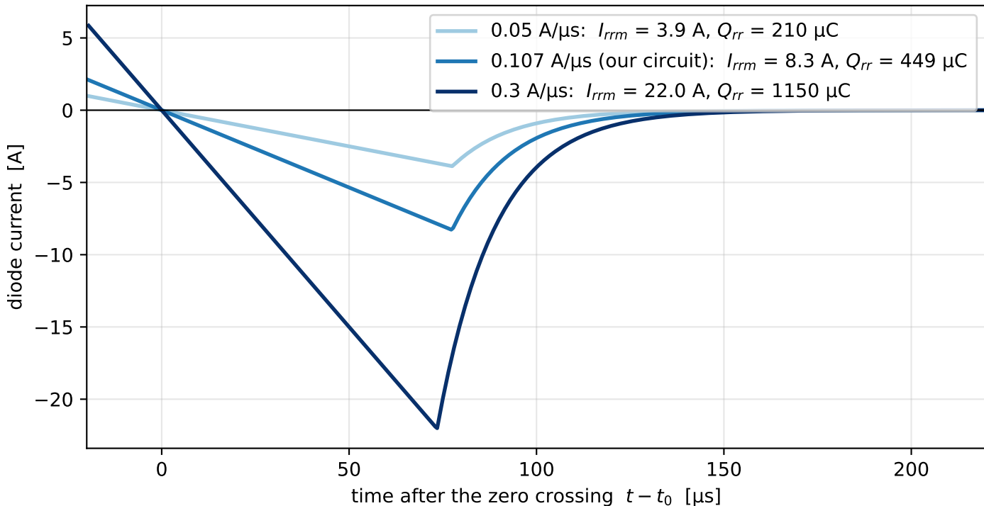
Same diode (same \tau and T_M ), three different slopes forced by the circuit
