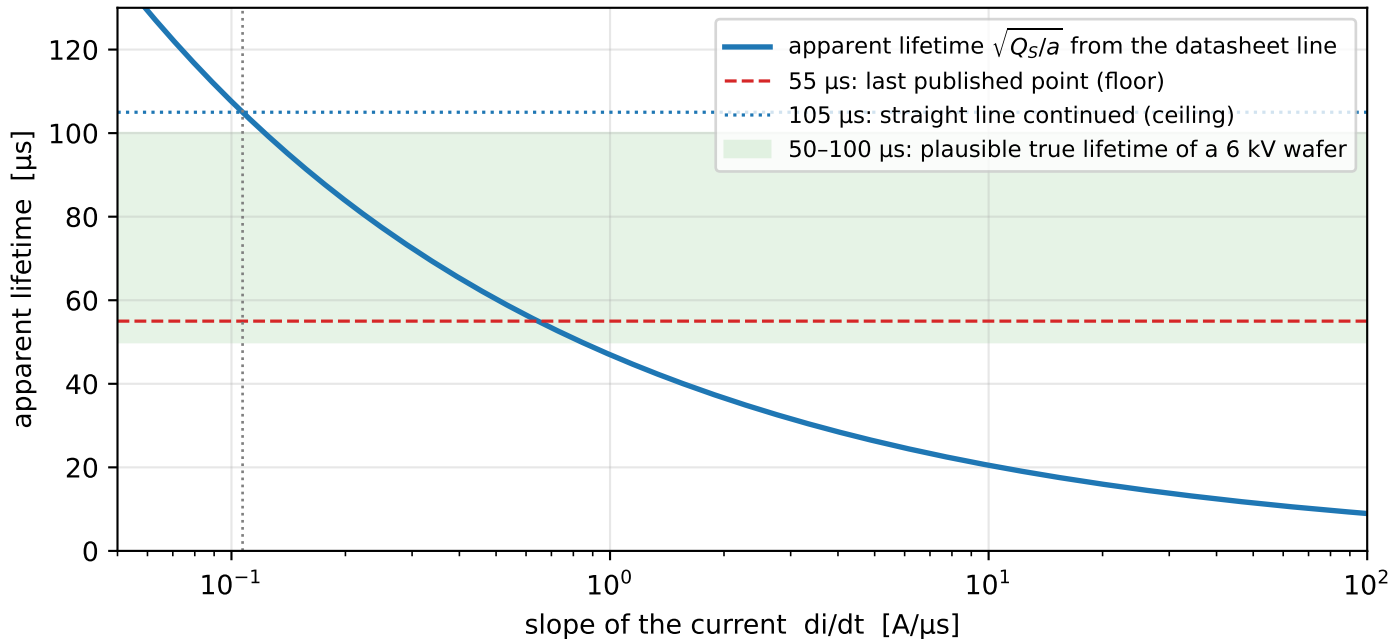
The lifetime you back out of the datasheet grows as the ramp gets slower
