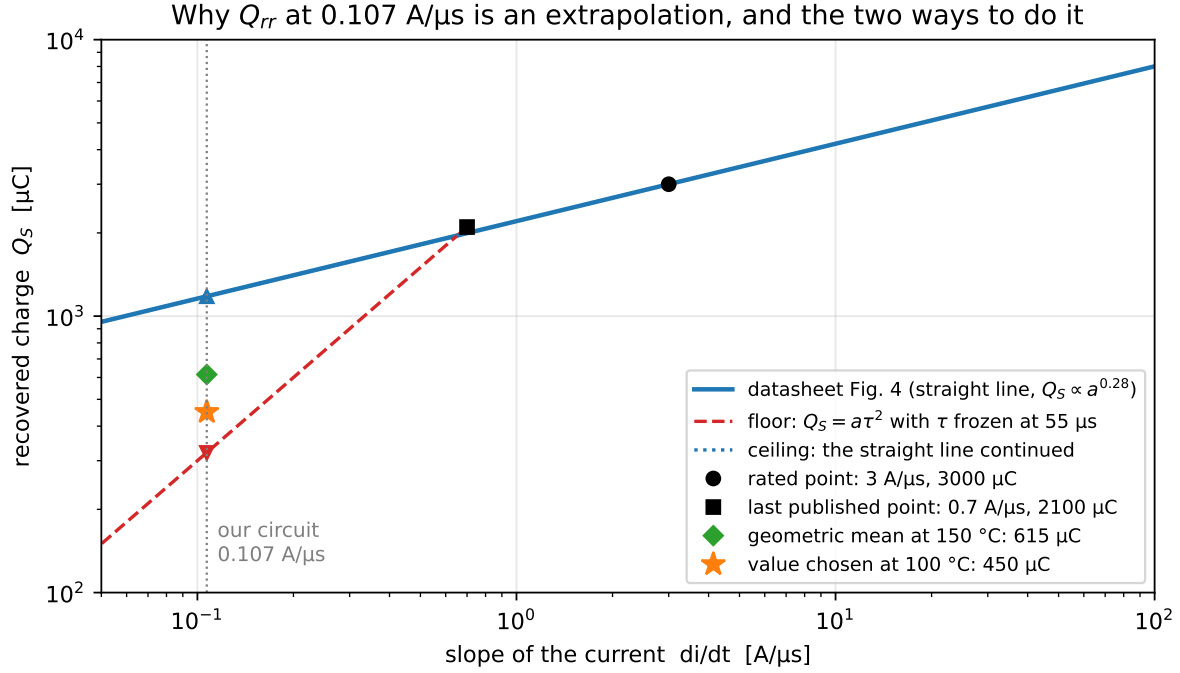
Figure 6: The datasheet line, the two extrapolations below the last published point, and the value chosen in the note. The vertical gap between floor and ceiling is a factor of 3.7 in charge, which is a factor of 1.9 in lifetime.
