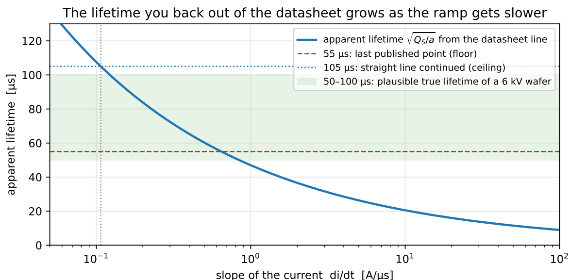
Figure 5: The lifetime you would deduce from the datasheet line at each slope. It cannot grow forever; it must level off at the real lifetime of the silicon. Where it levels off is what nobody knows without a measurement at 0.1 A/ \mu\text{s} .
