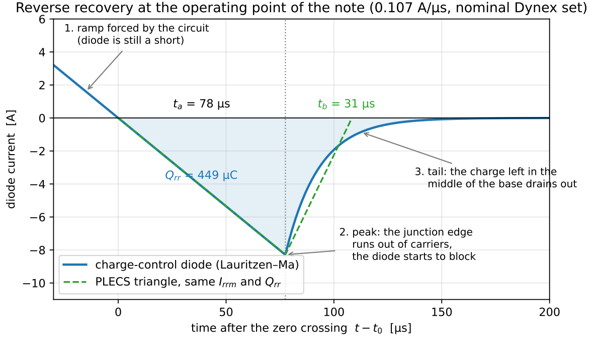
Figure 3: The recovery current at our operating point. Phase 1 is the ramp, forced by the circuit. Phase 2 is the peak, the moment the junction empties. Phase 3 is the tail. The dashed green line is the triangle PLECS uses in place of the real shape, with the same peak and the same area.
