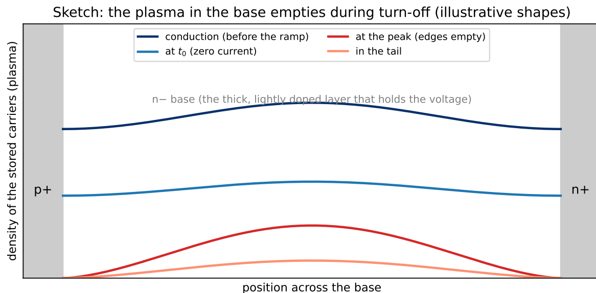
Figure 1: Sketch of the carrier density across the base at four moments of the turn-off. The shapes are illustrative. The important feature is that the cloud is removed from the edges inward, so the junctions run dry while there is still charge in the middle.
