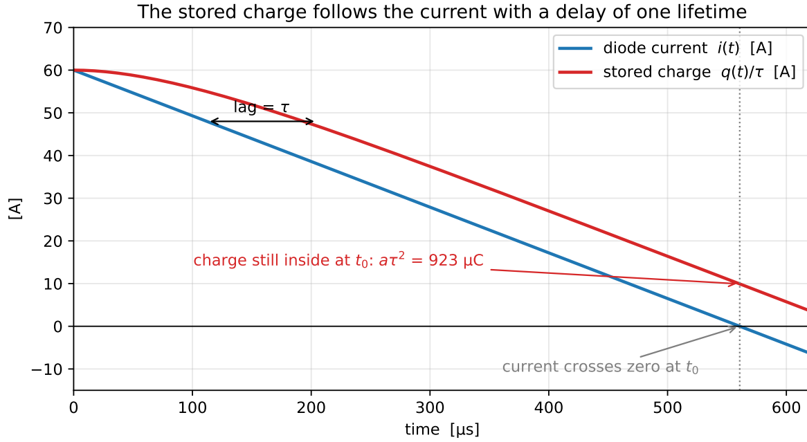
Figure 2: The diode current (blue) and the stored charge divided by the lifetime (red), on the same scale, during the 560 \mu\text{s} ramp of our rectifier. The red curve runs behind the blue one by one lifetime. When the current reaches zero, the charge is not zero: it is what the current was one lifetime ago, times \tau .
