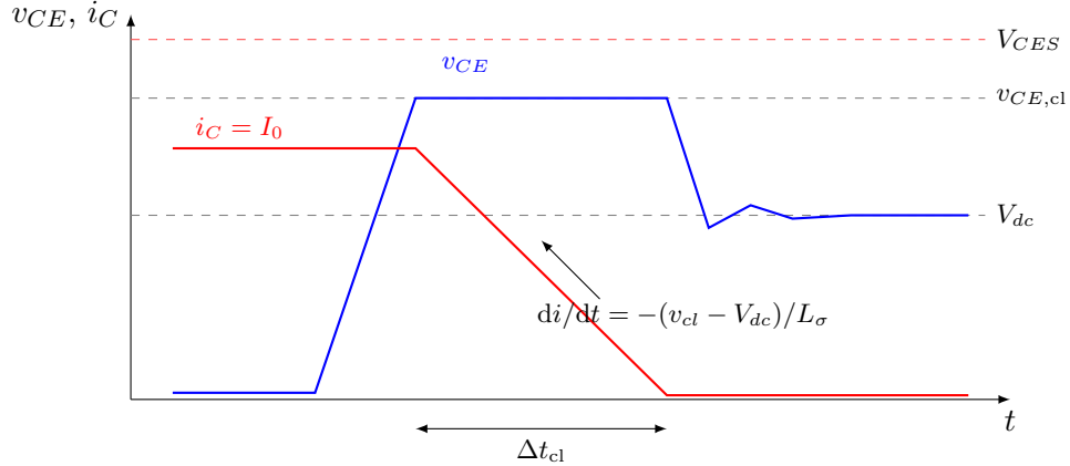
Figure 2: Idealised clamped turn-off. The voltage rises, is caught at v_{CE,cl} below the rating, and the current ramps down linearly during \Delta t_{cl} while the IGBT dissipates E_{IGBT} .
