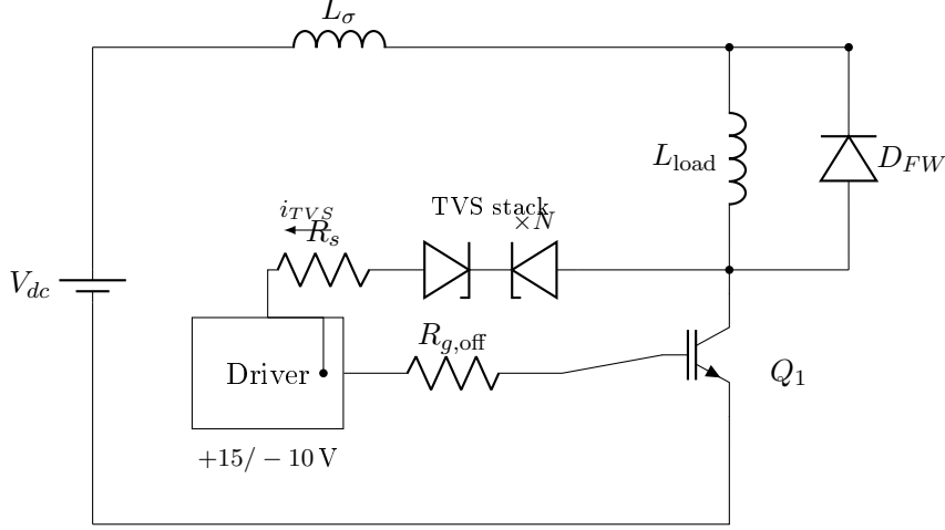
Figure 1: Basic active clamping of a low-side IGBT. The TVS stack (drawn as a bidirectional pair for one of the N devices) feeds the collector overvoltage back into the gate node; R_s is a small series/damping resistor. The stack should sense the auxiliary collector terminal to exclude the main-terminal inductance from the feedback path.
