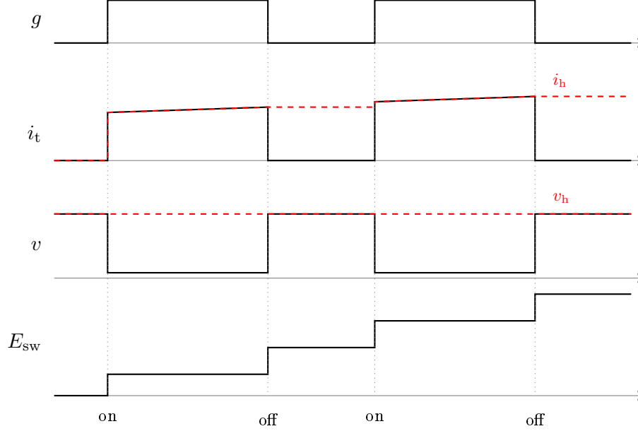
Figure 1: Sampling scheme. The held current i_h freezes at turn-off and is reused at the following turn-on; the held voltage v_h freezes at turn-on and is reused at the following turn-off. Each event adds a step to the cumulative energy E_{\text{sw}} .
