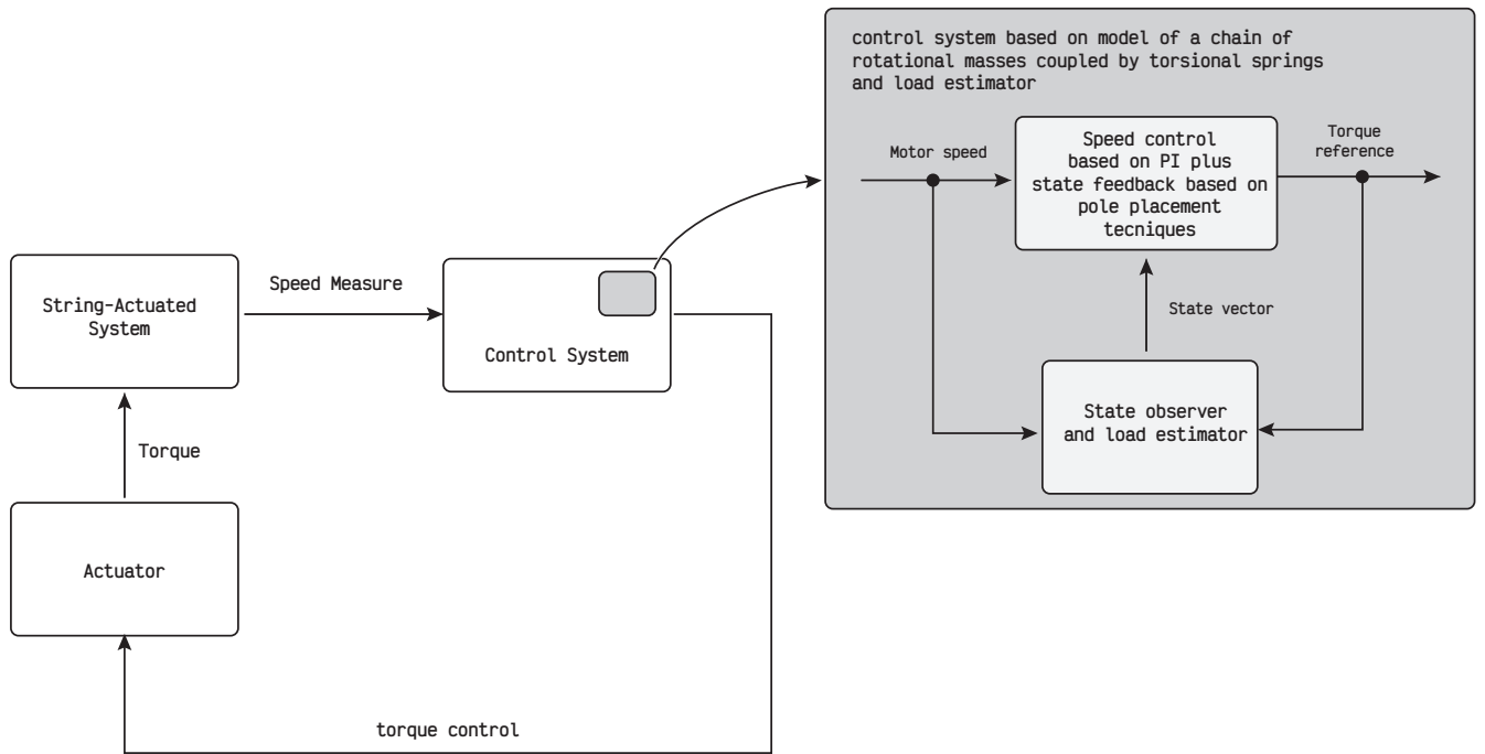
Figure 7: Conceptual control layout: speed control based on PI, pole placement and state observers.
