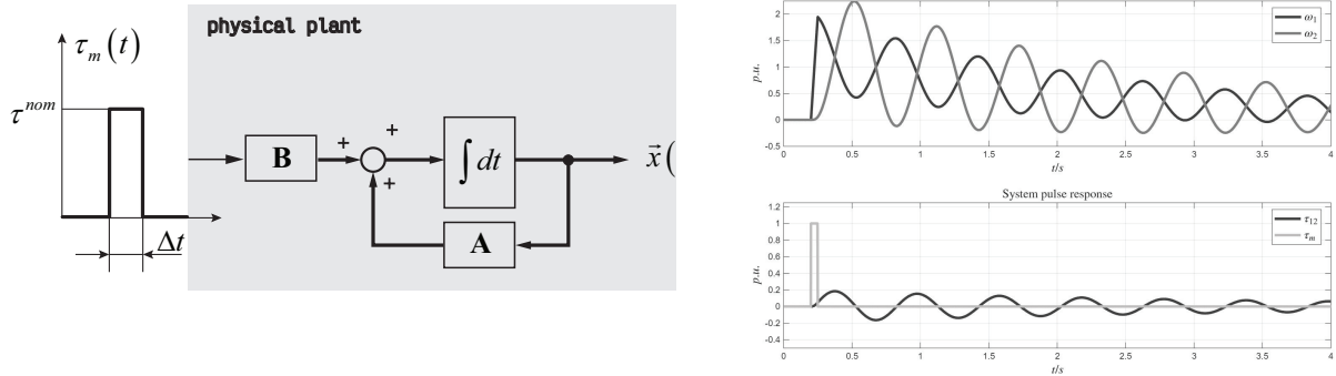
(a) Pulse test configuration system - open loop system.
