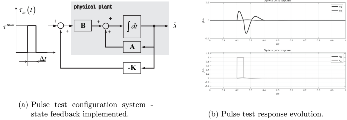
Figure 16: Pulse test analysis for the case of one dominant harmonic and with state feedback.
