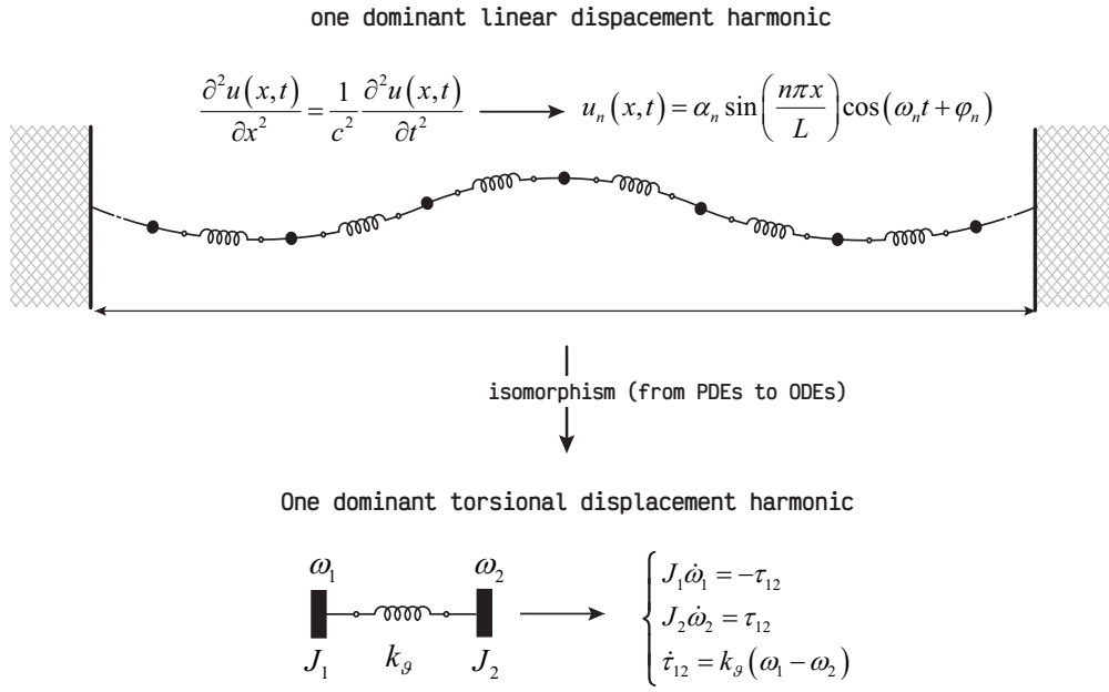
Figure 5: The dominant string oscillations are mapped onto a chain of harmonic oscillators to facilitate control design; here the case of one dominant harmonic.
