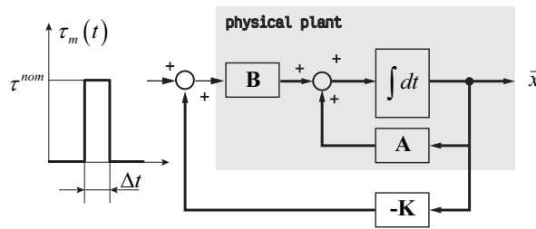
(a) Pulse test configuration system - state feedback implemented.
