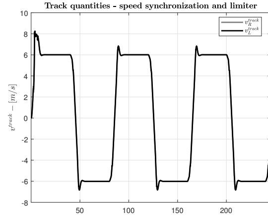
(b) Speed tracks synchronization and maximum speed limiter.
