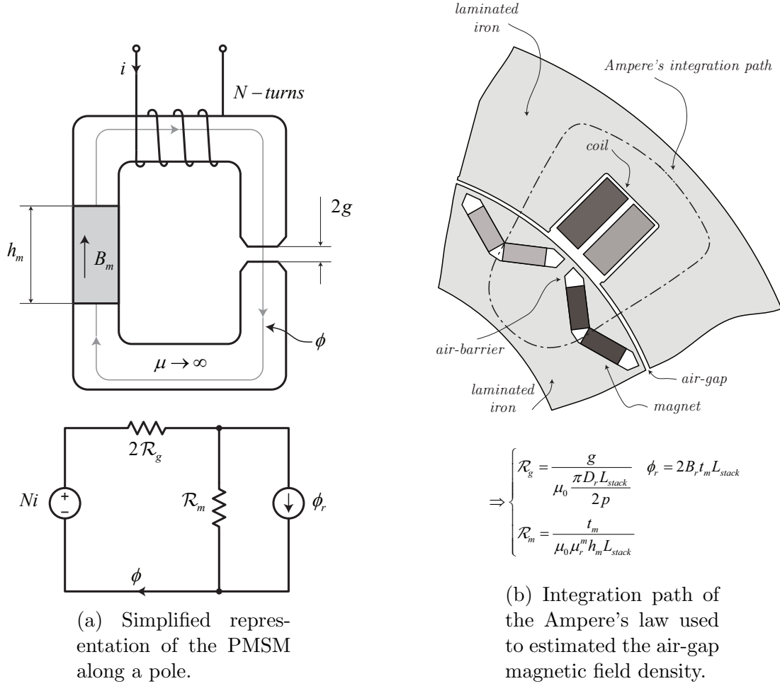
Figure 8.3: Magnetic circuit representation
