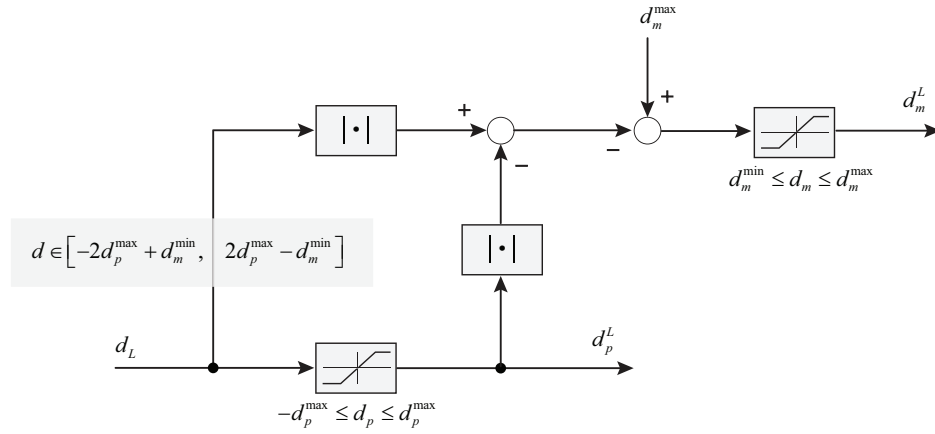
Figure 6.3: Total volumetric displacement for the left drive-line.
