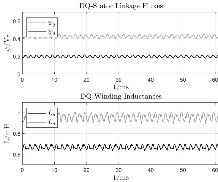
Figure 11.4: Simulation results: DQ-fluxes and DQ-inductances.
