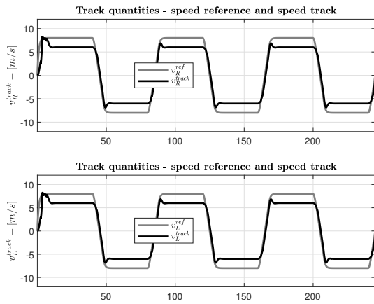
(a) Speed tracks tracking performance.
