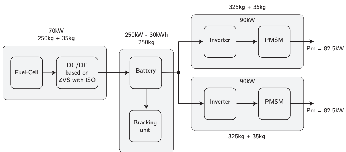
Figure 7.1: Electrical layout overview.
