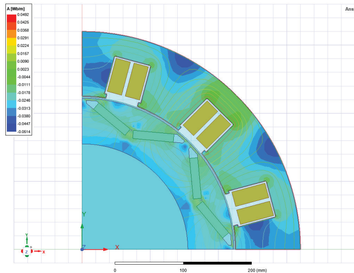
Figure 11.1: Magnetostatic analysis result.
