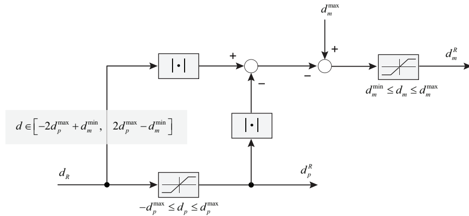
Figure 6.2: Total volumetric displacement for the right drive-line.
