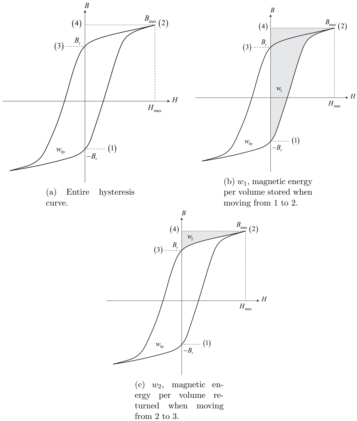
Figure 8.13: Determination of hysteresis loss.
