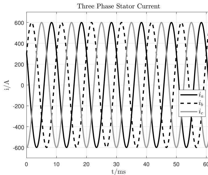
Figure 11.2: Simulation results: stator currents.
