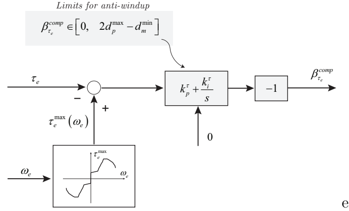
Figure 6.4: Engine anti-stall implementation.
