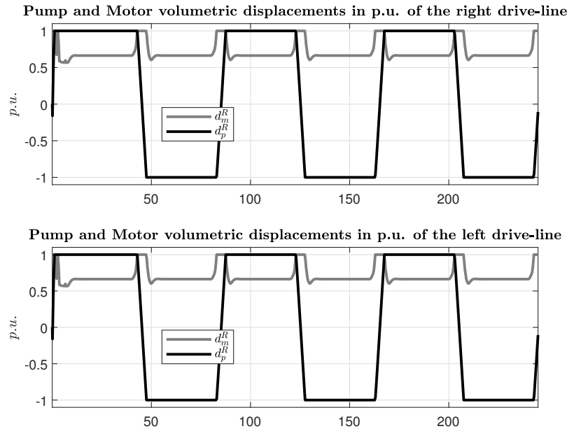
Figure 6.17: Volumetric displacements.
