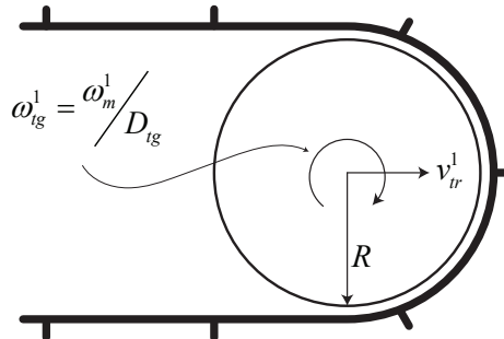
Figure 3.6: Track representation.
