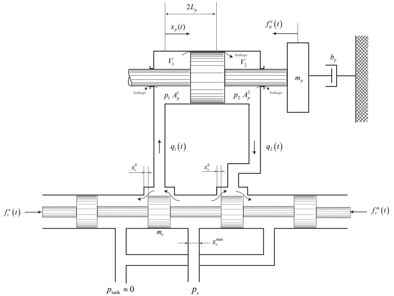
Figure 2.10: Four-way four-land valve bi-chamber piston system.
