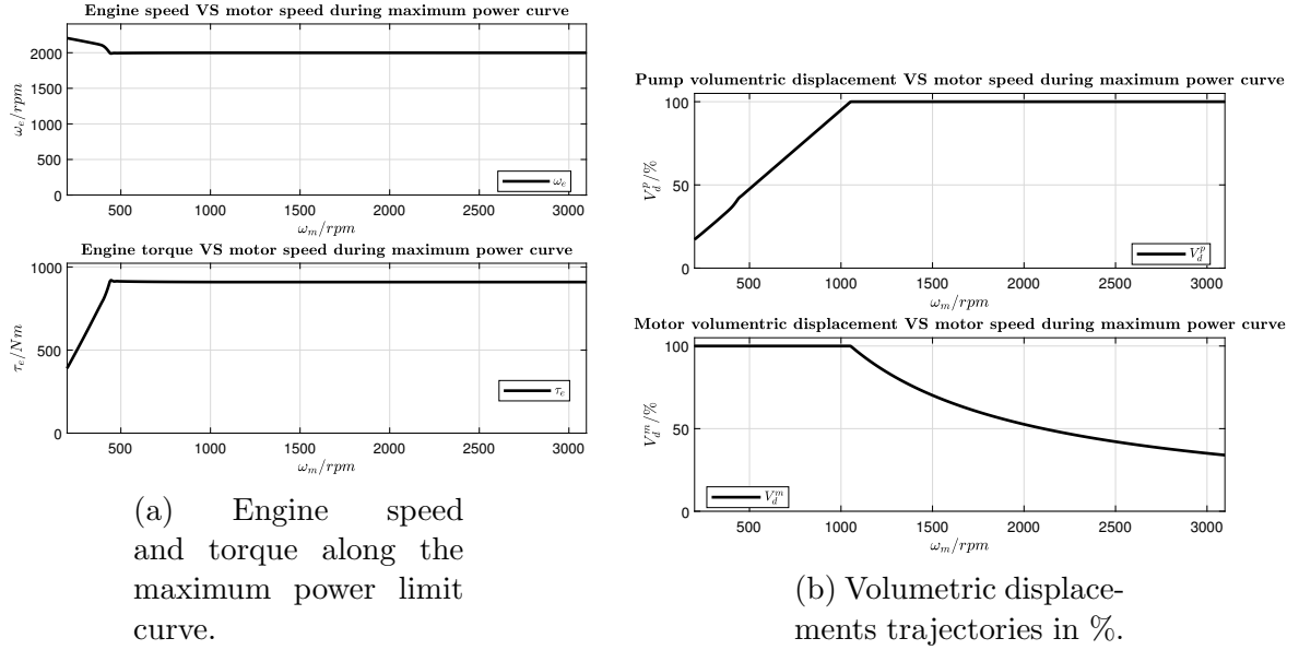
Figure 3.5: Power train limit curves - for one line.
