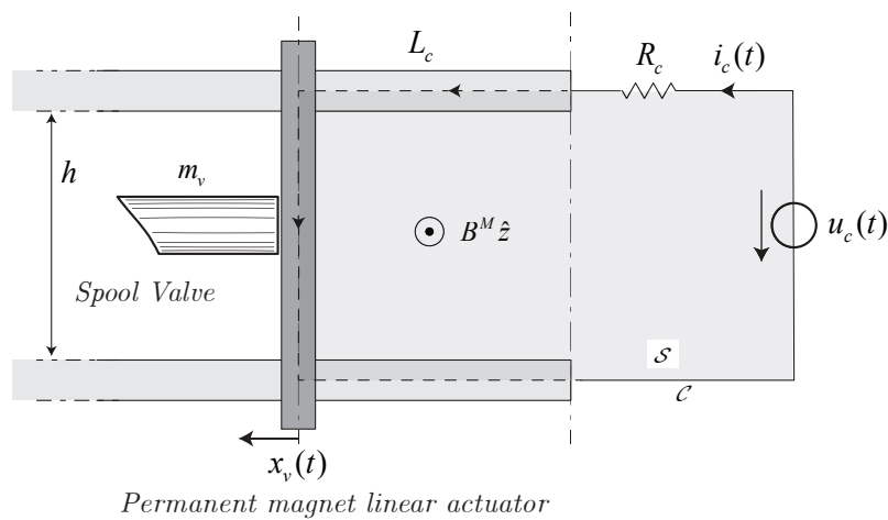
Figure 4.2: Permanent magnet spool valve actuator.
