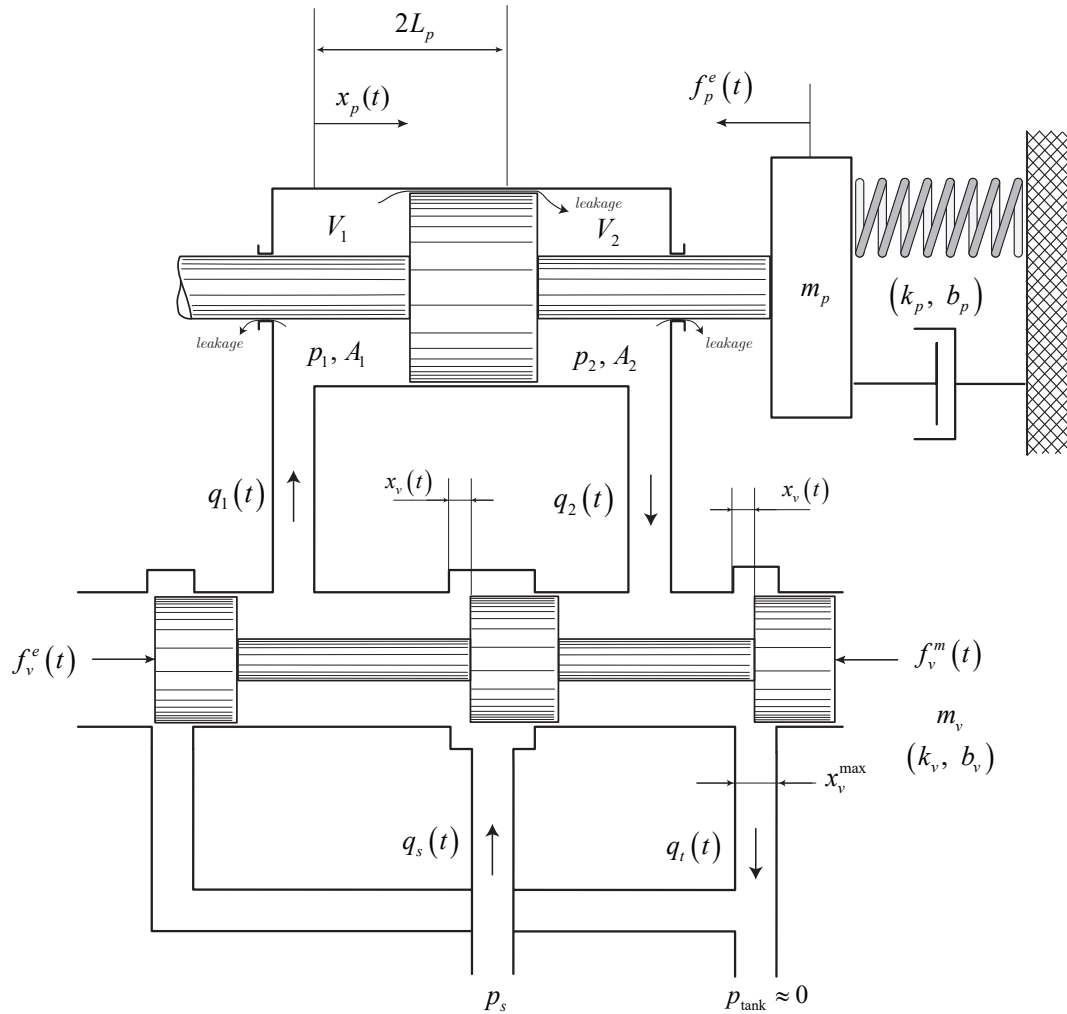
Figure 4.1: Four-way valve actuated piston during position changing.
