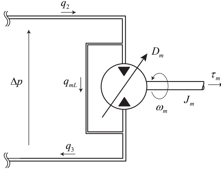
Figure 2.3: Hydrostatic motor.
