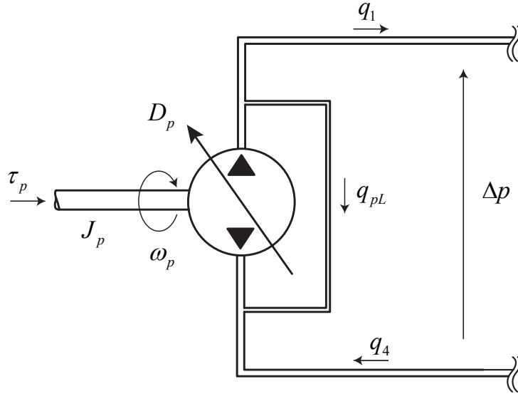
Figure 2.2: Hydrostatic pump.
