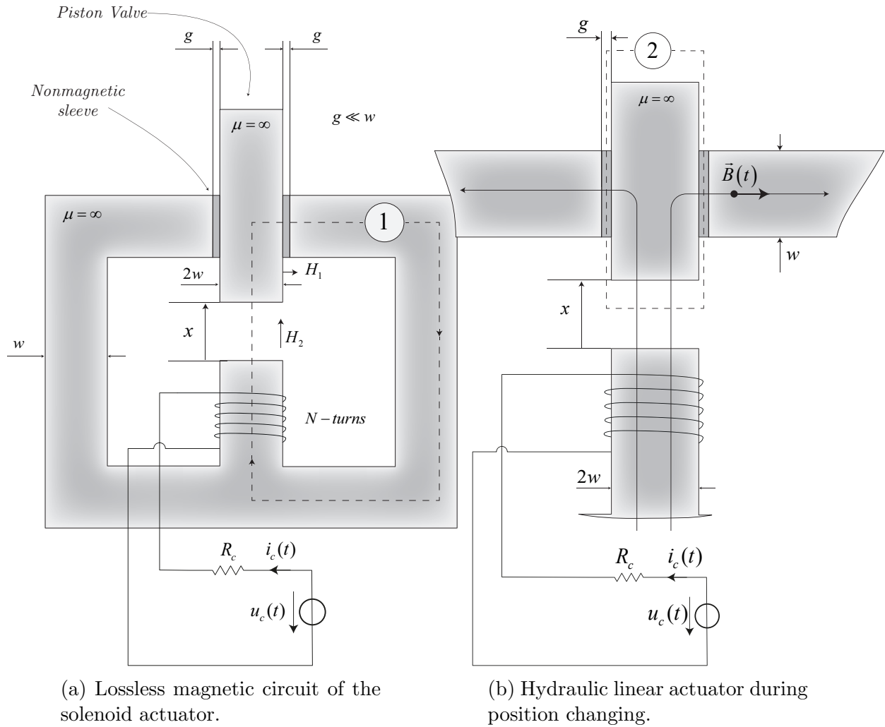
Figure 5.1: Solenoid actuator.
