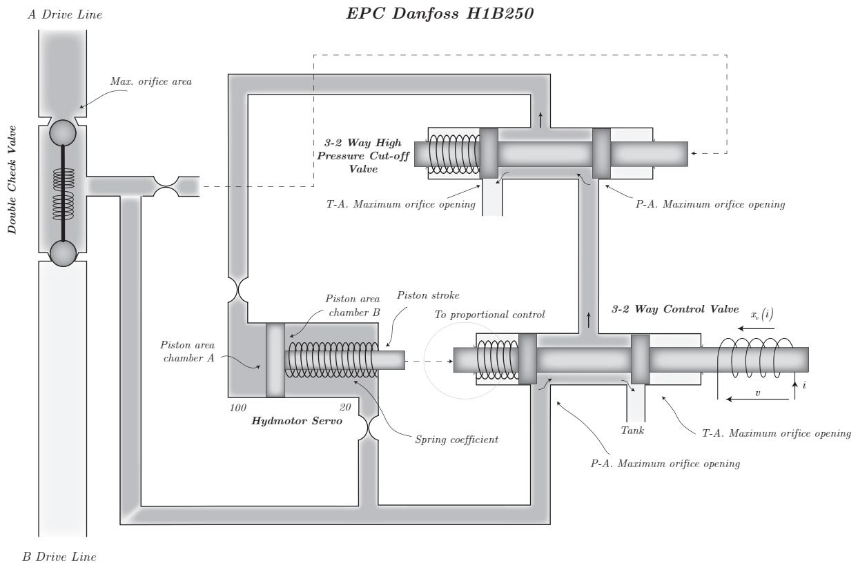
Figure 3.8: Motor servo layout.
