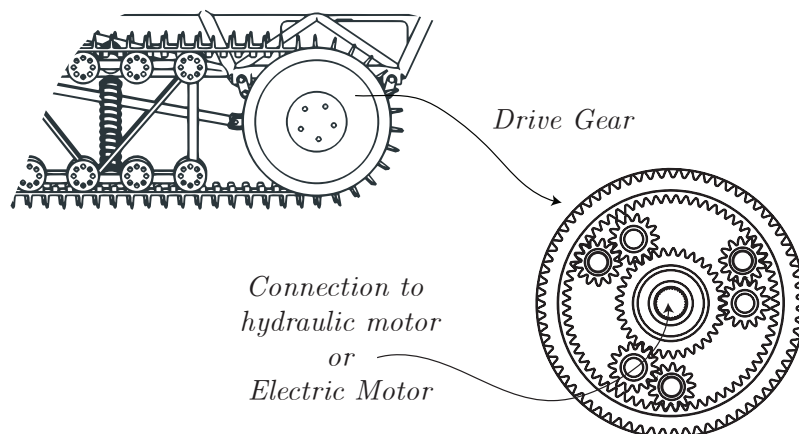
Figure 3.4: drive-gear representation.
