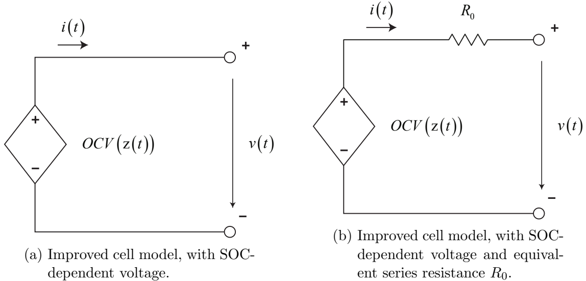
Figure 4: Equivalent circuit of the cell.
