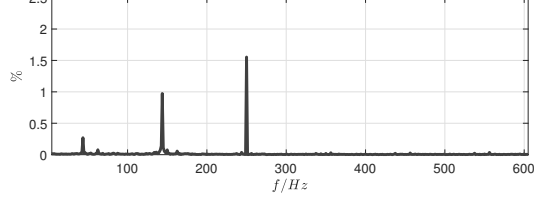
Four modules - grid phase current spectrum 2 \leq h \leq 11 at rated operating point - I_{oc} = 50kA
