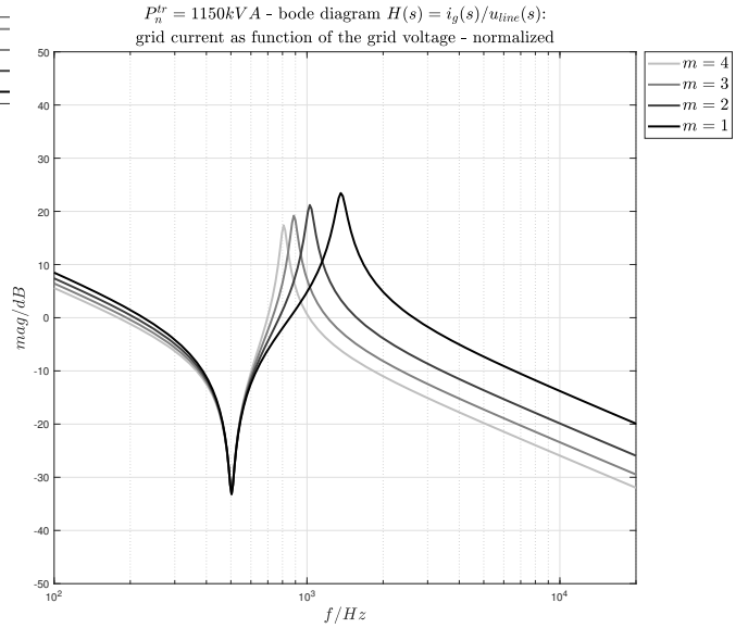
(b) Bode diagram of the equivalent of the transfer function: i_g(s)/u_{line}(s) , for m = 1, 2, 3, 4 modules connected to the grid via a transformer of P_n = 1150\text{ kVA} .
