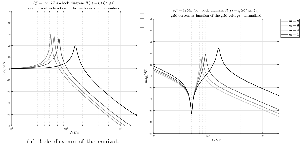
(b) Bode diagram of the equivalent of the transfer function: i_g(s)/u_{line}(s) , for m = 1, 4, 6, 8 modules connected to the grid via a transformer of P_n = 1850 \text{ kVA} .
