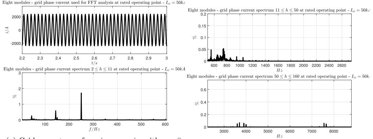
(a) Grid current waveform i_{line} = n \cdot i_g , with n = 8 (top), and spectrum analysis of the grid current (bottom). The components related to the 5th PSM harmonic distortion are visible at frequency of 43.6 Hz, and 143.6 Hz, while the residual current harmonic distortion correlated to the 5th harmonic grid voltage is visible at frequency of 250.0 Hz.
