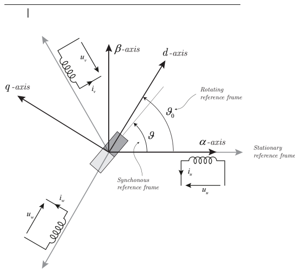
Figure 25: Reference frames
