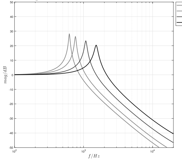
(a) Bode diagram of the equivalent of the transfer function: i_g(s)/i_s(s) , for m = 1, 2, 4, 6 modules connected to the grid via a transformer of P_n = 1670\text{kVA} .
