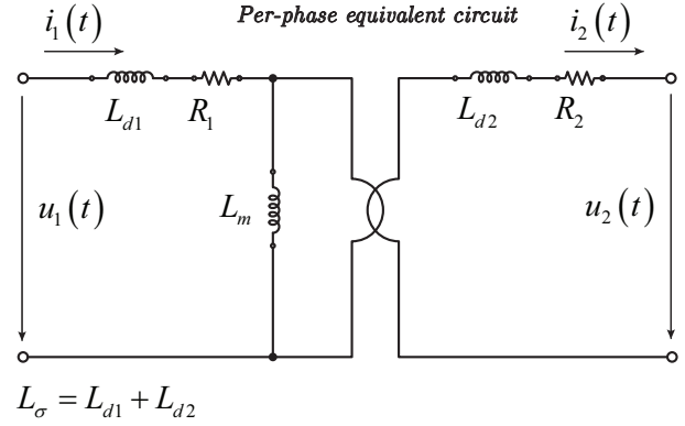
(b) Per-phase equivalent circuit of the MV/LV transformer.
