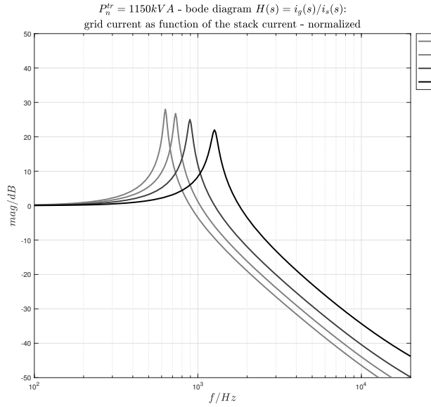
(a) Bode diagram of the equivalent of the transfer function: i_g(s)/i_s(s) , for m = 1, 2, 3, 4 modules connected to the grid via a transformer of P_n = 1150\text{ kVA} .
