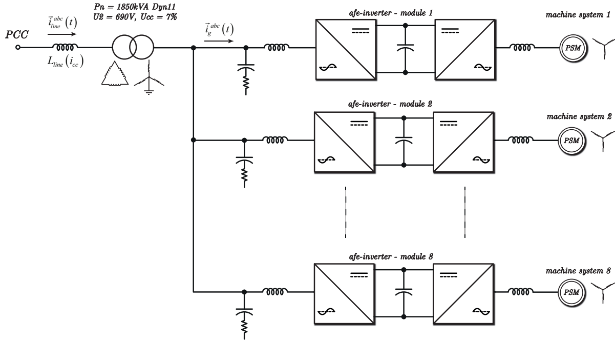
Figure 40: Functional representation of the 1.65MW power solution.
