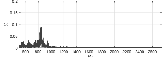
Three modules - grid phase current spectrum 50 \leq h \leq 160 at rated operating point - I_{ce} = 50k
