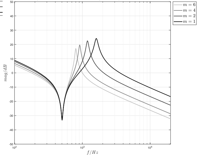
(b) Bode diagram of the equivalent of the transfer function: i_g(s)/u_{line}(s) , for m = 1, 2, 4, 6 modules connected to the grid via a transformer of P_n = 1670\text{kVA} .
