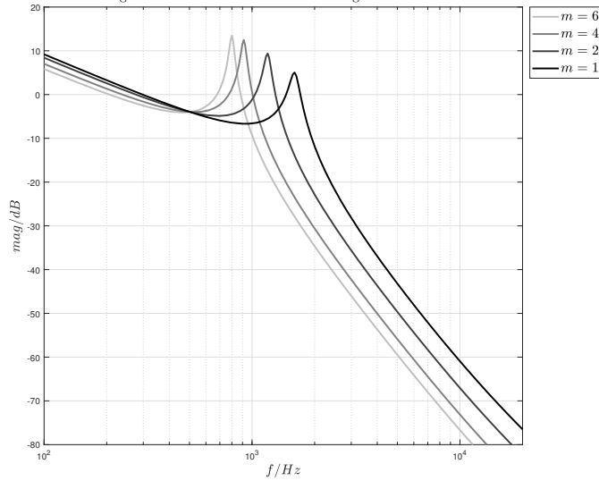
(c) Bode diagram of the equivalent of the transfer function: i_g(s)/u_s(s) , for m = 1, 2, 4, 6 modules connected to the grid via a transformer of P_n = 1670\text{kVA} .
