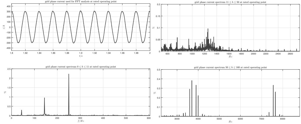
(a) grid phase current (top); grid phase current spectrum (bottom); components at 43.6 Hz and 143.6 Hz are coupled to the fifth harmonic component of the PSM back EMF; component at 250 Hz is coupled to the homologous grid voltage harmonic component.
