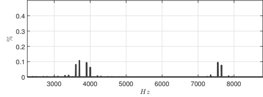
Three modules - grid phase current spectrum 50 \leq h \leq 160 at rated operating point - I_{ce} = 50k
