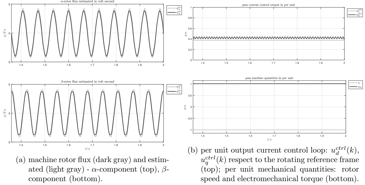
Figure 19: inverter side per unit quantities, during nominal power condition for a single ElectricalDrive connected to a i_{cc} = 50 kA grid with MV/LV transformer with a nominal power of P_n = 1150 kVA.
