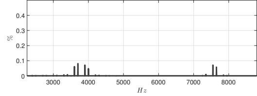
Four modules - grid phase current spectrum 50 \leq h \leq 160 at rated operating point - I_{oc} = 50kA
