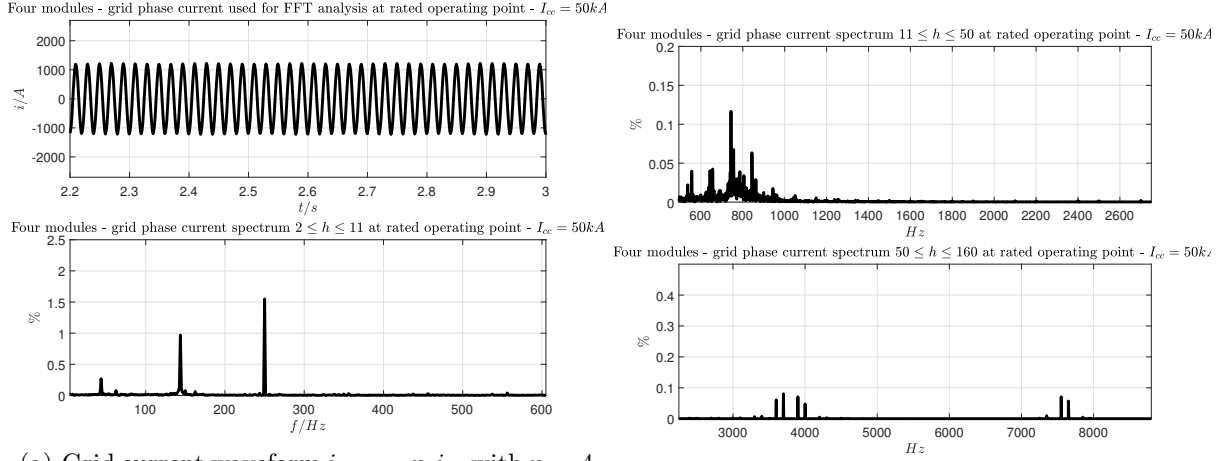
(b) Grid current spectrum analysis; effects of the resonance are visible (top) around the frequency f_0 = \frac{1}{2\pi\sqrt{L_{grid} \cdot n \cdot C_{Fu}}} , where L_{grid} = L_{line} + L_{\sigma} ; residual grid current harmonics related to the PWM modulation are also visible (bottom).
