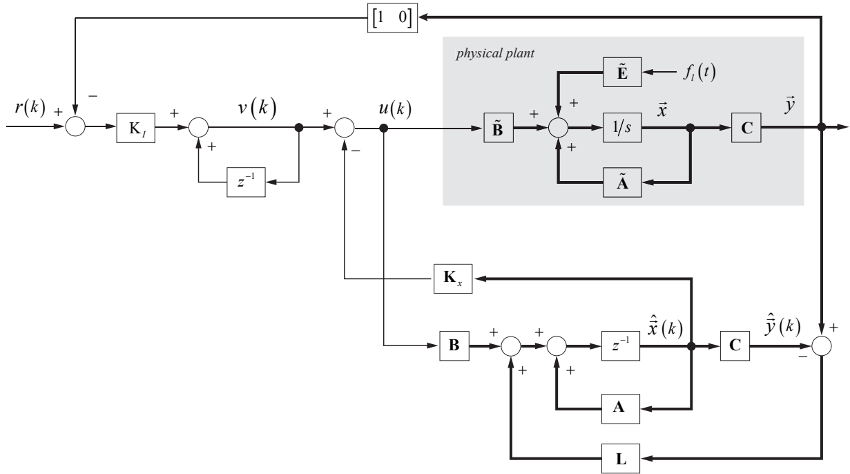
Figure 5: Control architecture.
