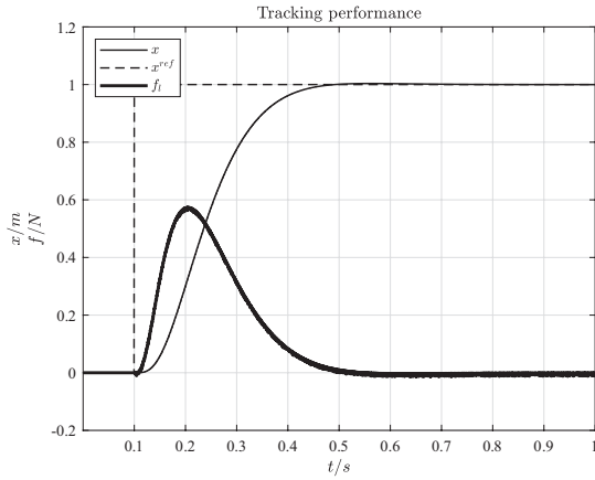
(a) Tracking performance for a given position set-point. The position reference x^{ref} is in dashed. Case (1).
