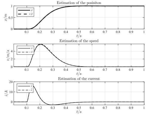
(b) Observer performance. Case (1).
