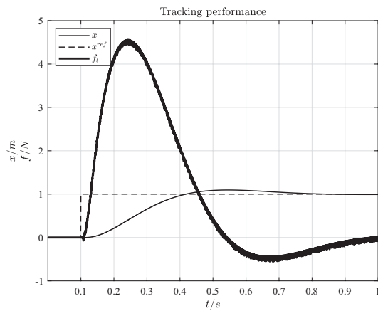
(a) Tracking performance for a given position set-point. The position reference x^{ref} is in dashed. Case (2).
