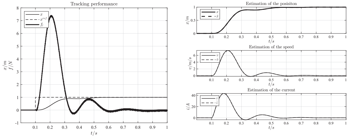
(a) Tracking performance for a given position set-point. The position reference x^{ref} is in dashed. Case (2).
