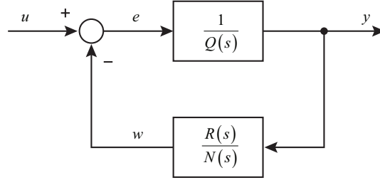
Figure 5.1: Feedback representation of H(s) .
