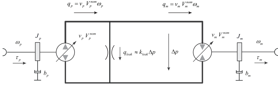
(a) Hydrostatic driveline layout with internal leakage which emulates the volumetric efficiency of the driveline.
