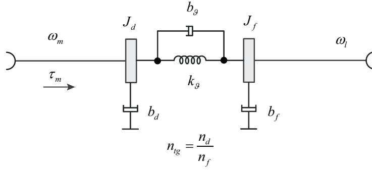
(b) End gear transmission of the hydrostatic transmission.
