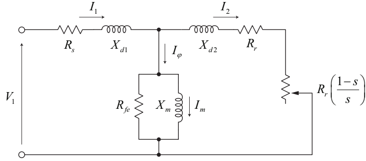
Figure 4.3: IM equivalent circuit.
