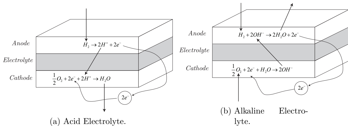
Figure 5: Schematic diagram of different fuel cells
