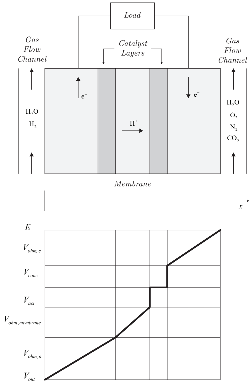
Figure 3: Schematic diagram of a PEM fuel cell and voltage drop across it.
