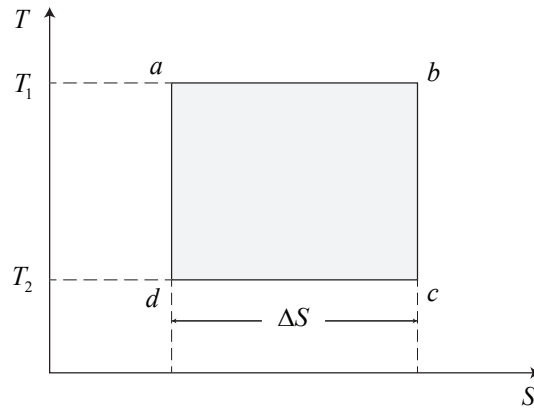
Figure 7: Temperature-entropy diagram for a Carnot cycle.
