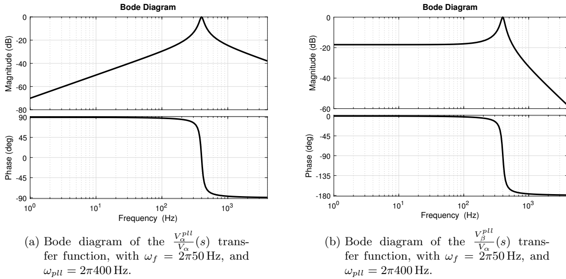
Figure 11: Bode diagram of the QSG-PLL based on direct and inverse Parck transform.
