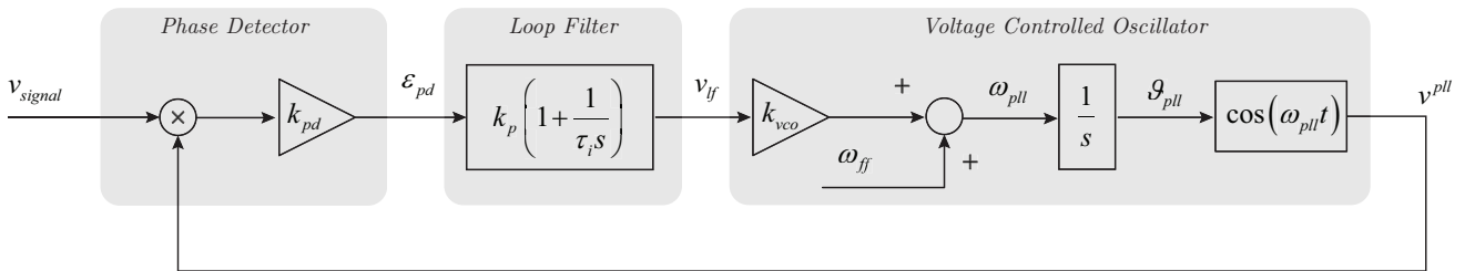
Figure 2: Block diagram of an elementary PLL .
