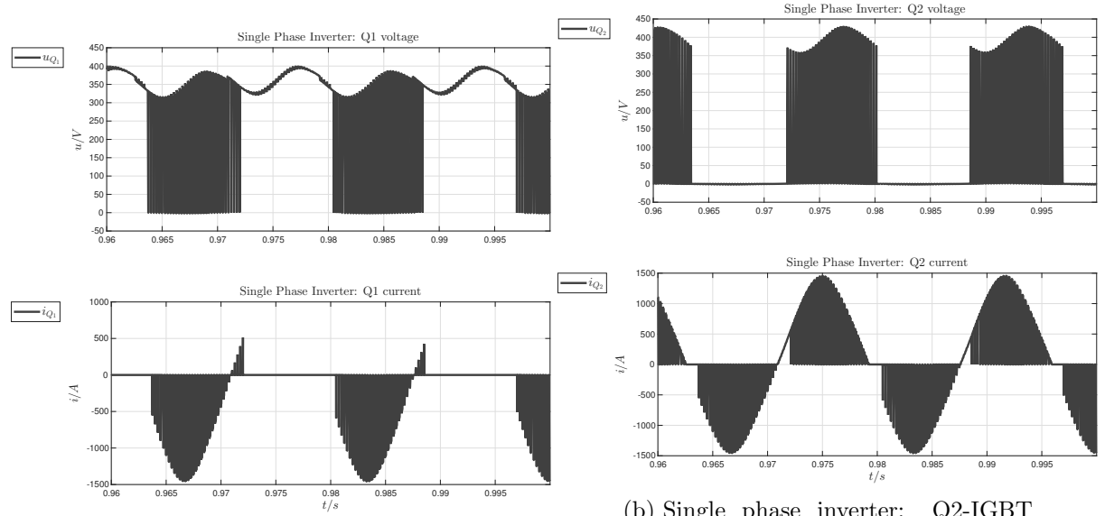
(a) Single phase inverter: Q1-IGBT voltage and current. The aim of this image is to proof the effective operative working of the three level NPC single phase inverter.
