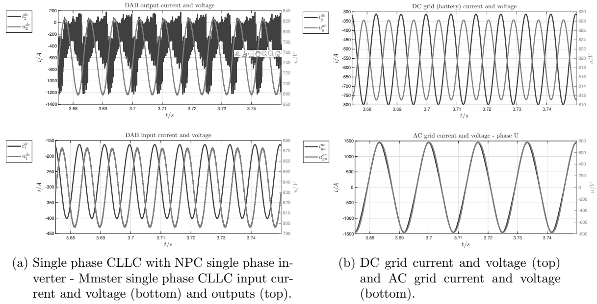
Figure 22: Single phase CLLC with NPC single phase inverter - performance of two stages single phase SST: single phase CLLC input/output and grids.
