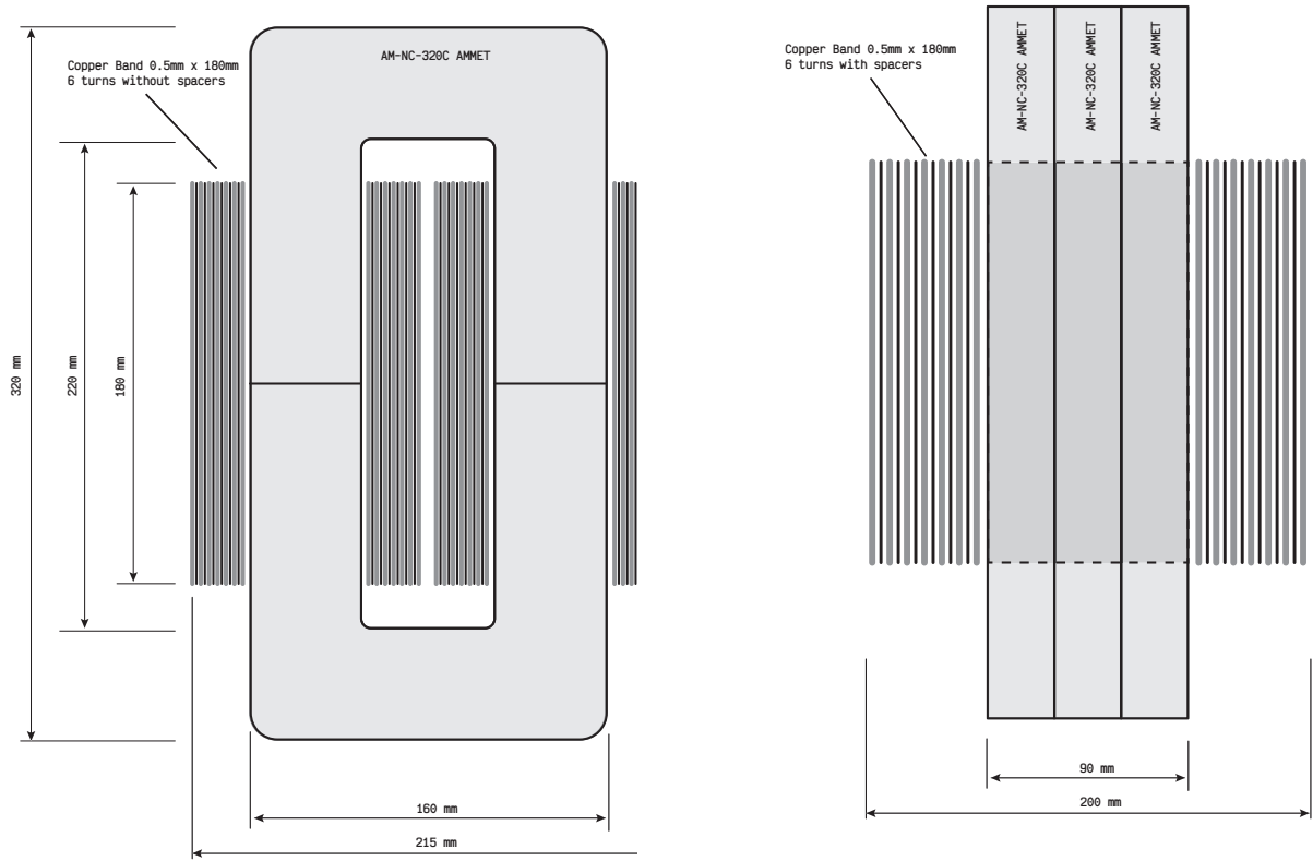
(a) Single phase transformer for the three-phase DAB - front view.
