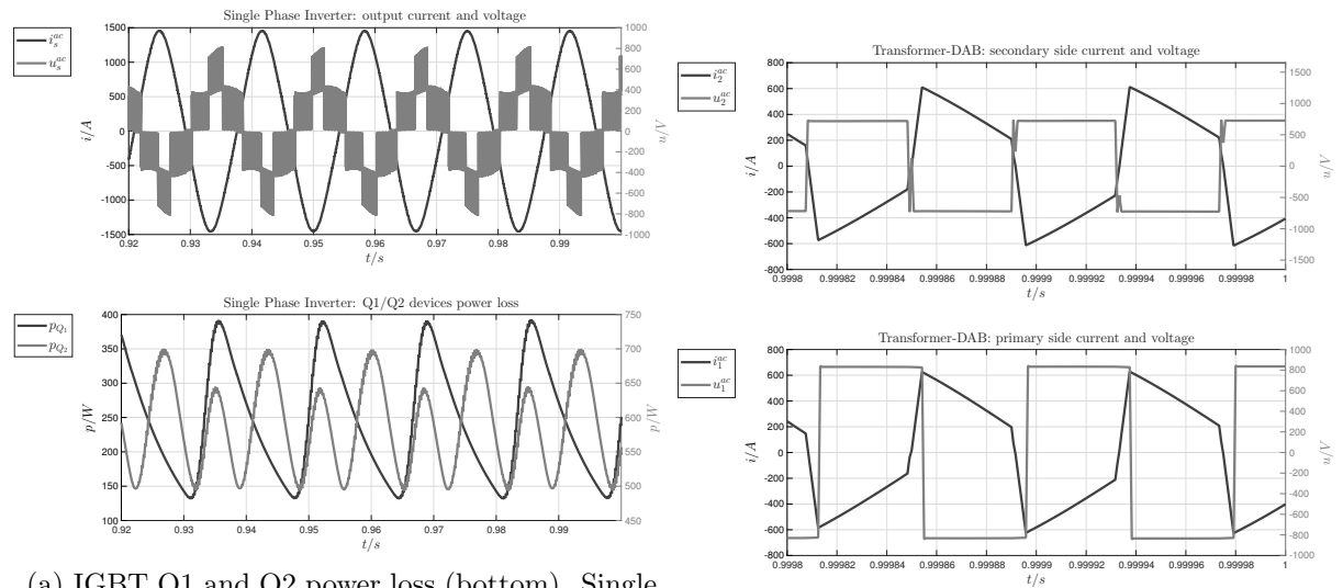
(b) Single phase DAB operative condition at nominal flow power.
