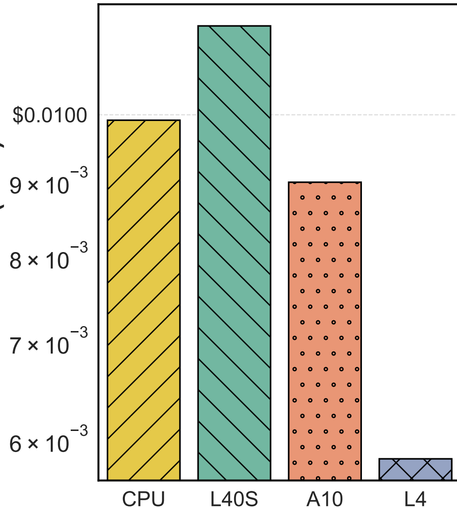
(b) Total Workload Cost
