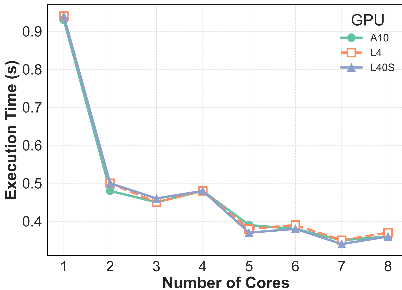
(a) Q2: Execution Time vs CPU Cores
