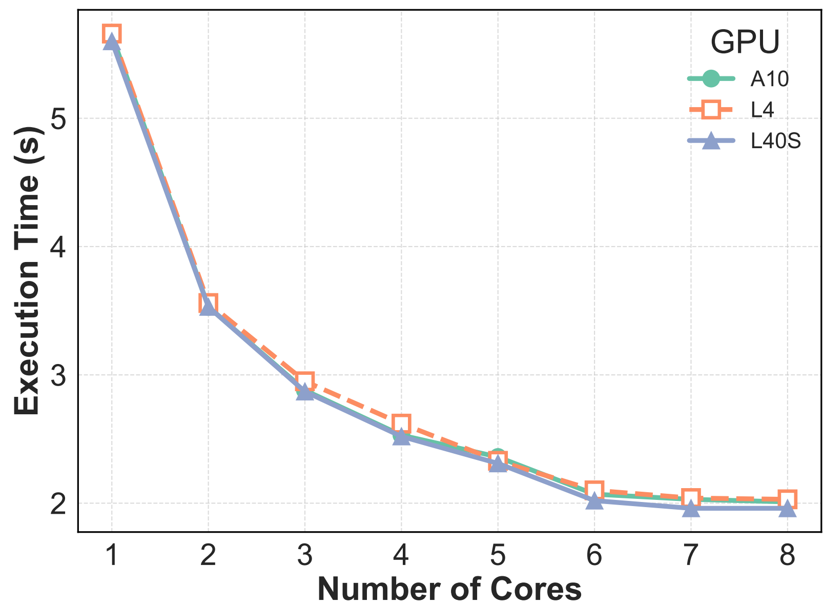
(b) Q11: Execution Time vs CPU Cores
