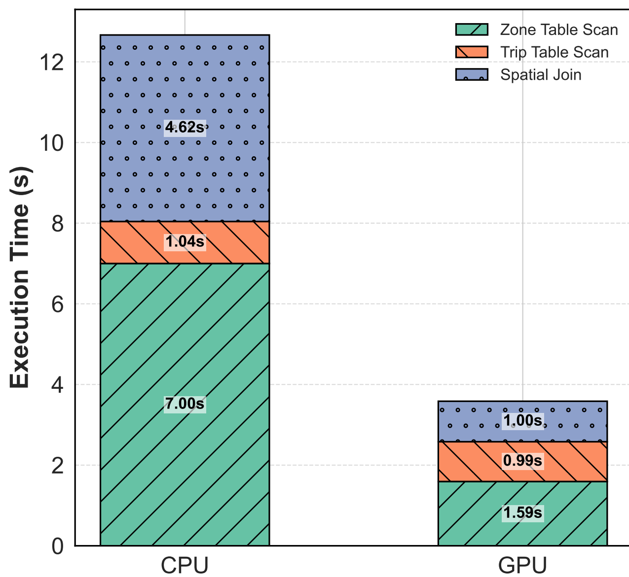
(a) Q2: CPU vs GPU Execution
