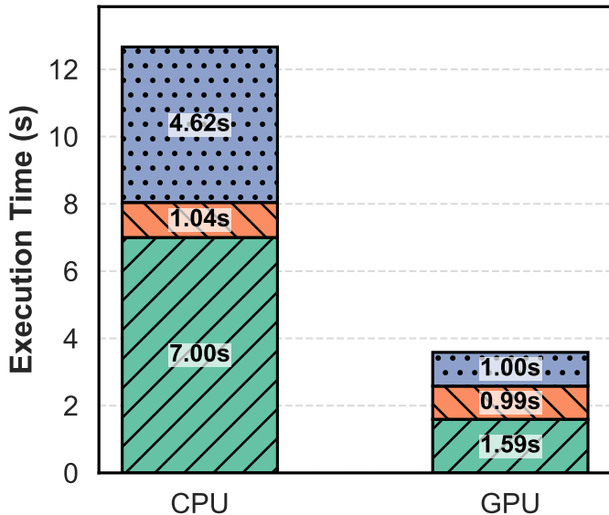
(a) Q2: CPU vs GPU
