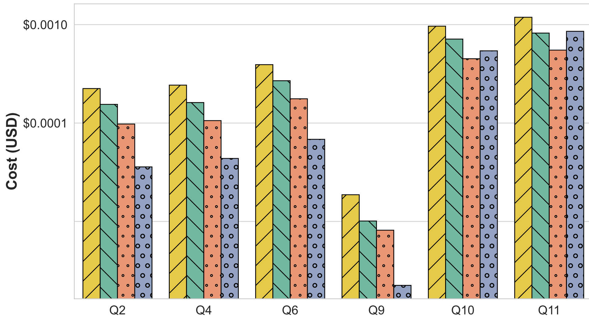
(a) Cost per Individual Query
