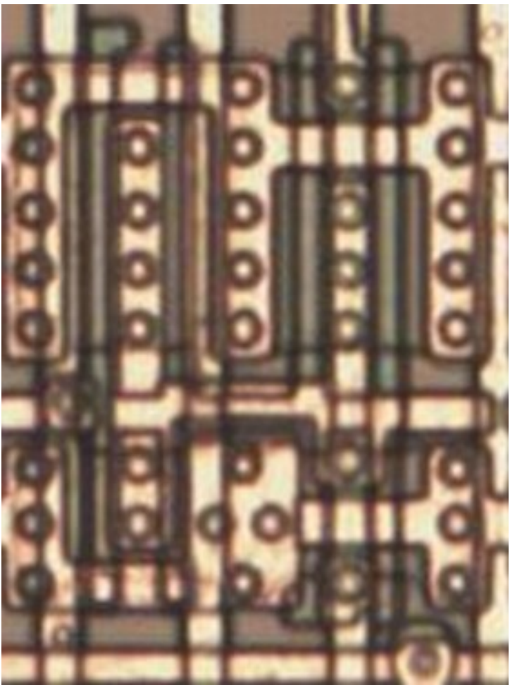
Same cell on LA32 (MB87136A)
