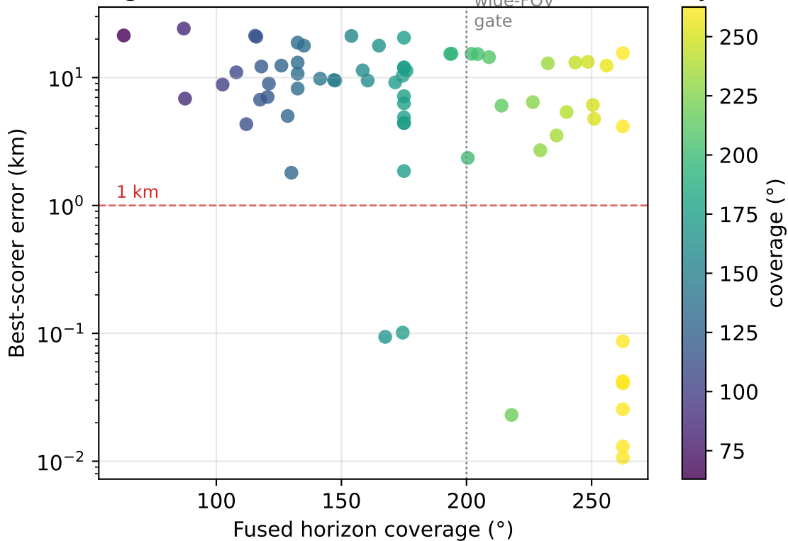
Coverage of the fused horizon vs achievable accuracy
