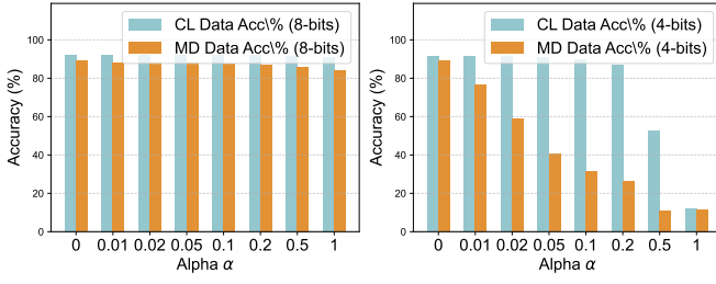
Fig. 2: The performance of the model under different values of \alpha in the modified objective function. The bluish-gray and yellow bars represent the accuracy of clean data and modified data, respectively.
