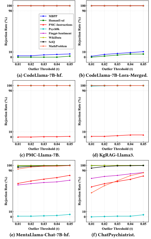
Figure 5: Ablation results based on outlier thresholds ( t ).
