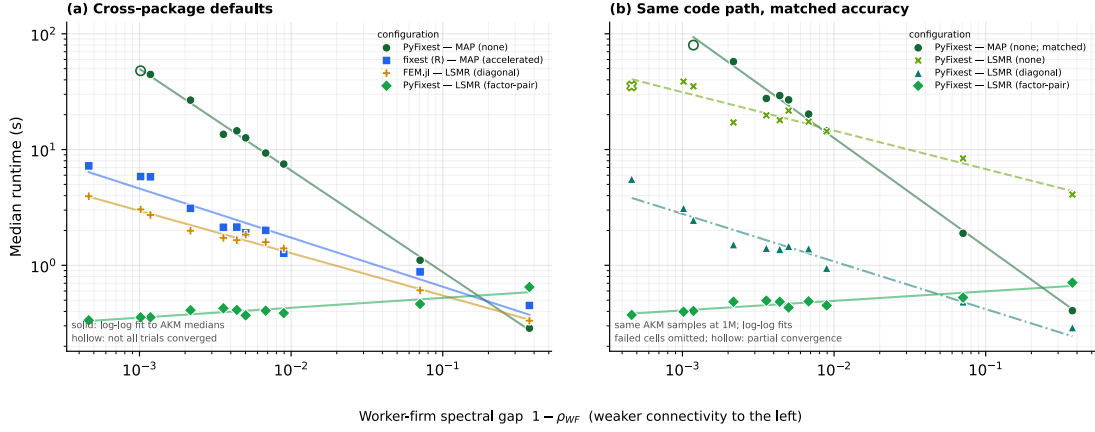
Figure 5: Runtime against the worker-firm spectral gap, log-log, on common axes. Both panels show the controlled 1M-observation AKM sweep; every marker uses the same stored sample for its scenario. Solid lines are log-log fits to the AKM medians. Panel (a) compares package defaults. Panel (b) reruns the PyFixest configurations on the same samples at matched accuracy under a shared iteration cap. Failed cells are omitted, and hollow markers denote partial convergence.
