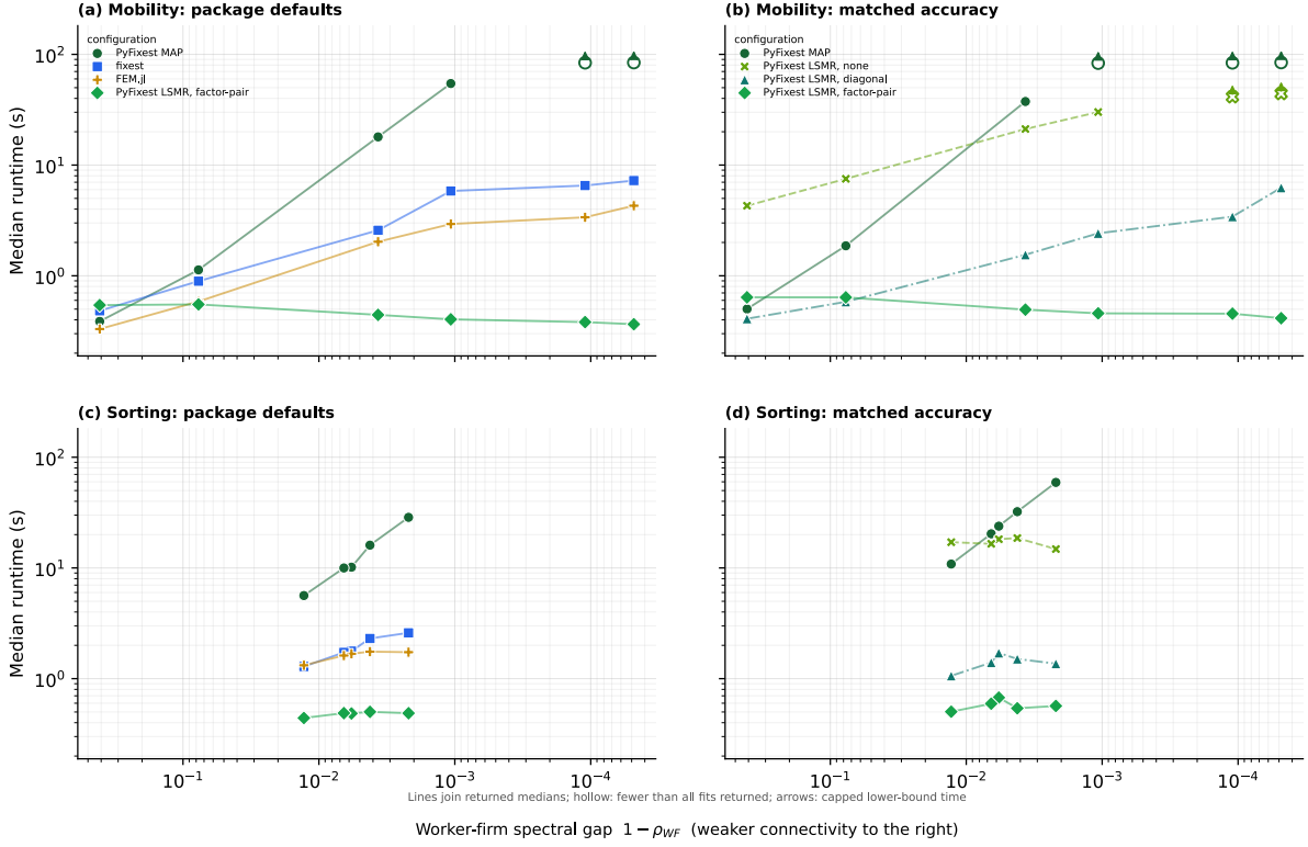
Figure 1: Median full-regression runtime against the worker-firm spectral gap, on log-log axes. Smaller gaps mean weaker connectivity, so the horizontal scale decreases from left to right. All four panels use the same horizontal scale. The top row varies worker mobility and the bottom row varies sorting among movers in simulated worker-firm-year panels with 1 million observations. The left column uses package defaults; the right column fixes the PyFixest code path and uses tolerances selected for comparable achieved accuracy. Packages apply their own default singleton treatment in the left column. Filled markers report the median from a complete three-fit cell; hollow markers report a returned median from fewer than three fits. Lines join returned medians for each configuration in spectral-gap order; they are not fitted trends. Arrows show the median elapsed time of capped fits as a lower bound and are not connected. Non-cap failures are omitted.
