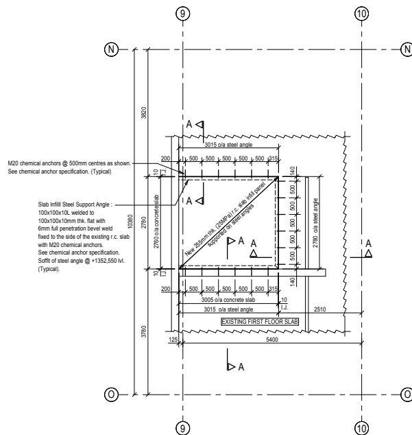
PLAN R.C. SLAB INFILL PANEL ON EXISTING FIRST FLOOR
