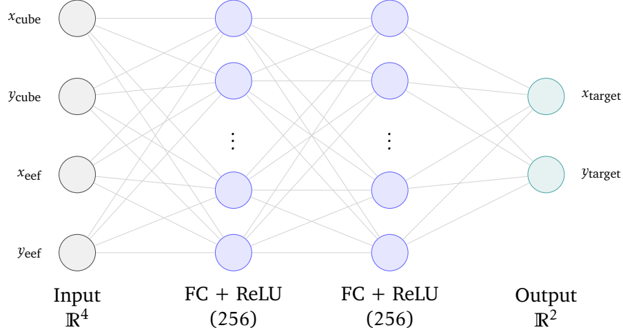
Figure 1: MLP policy architecture shared by SAC and TD3.
