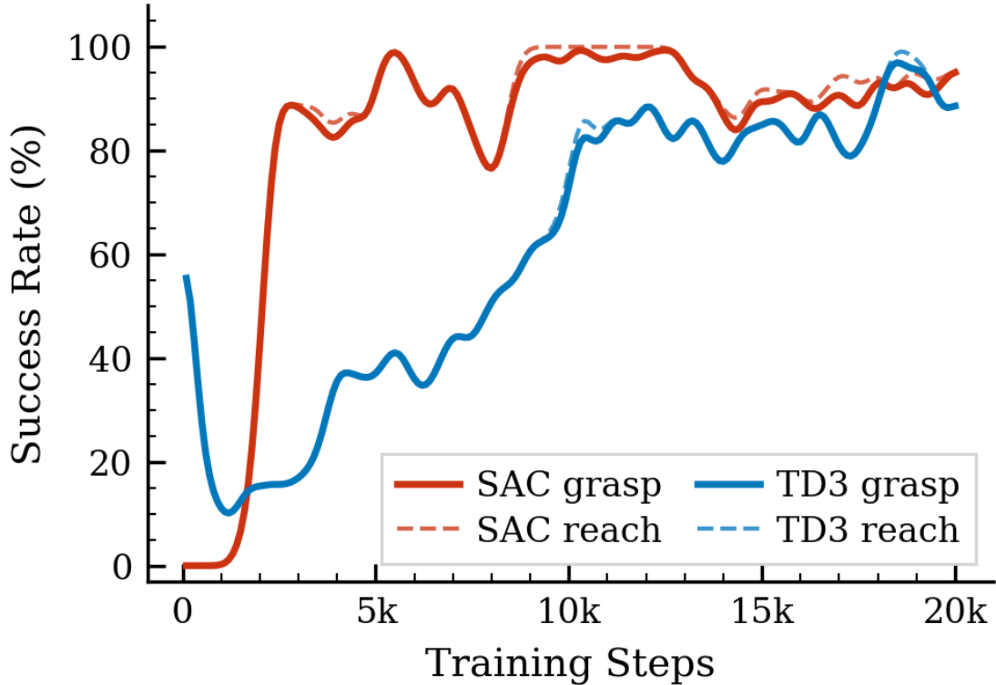
Figure 4: Rolling grasp success rate during training.
