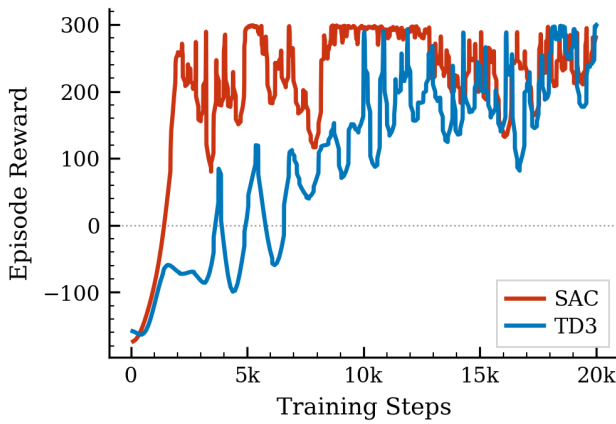
Figure 2: Episode reward during training.
