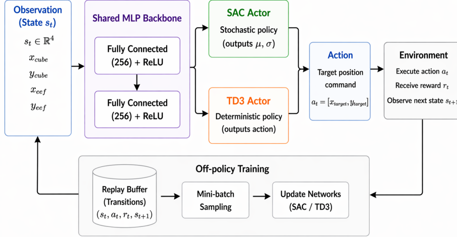
Figure 1: Overall training framework.
