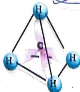
Fig. 13.1 Structure of methane
