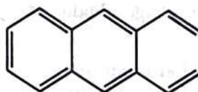
Anthracene
