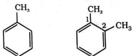
Methylbenzene (Toluene)
