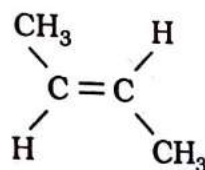
trans-But-2-ene (b.p. 274 K)
