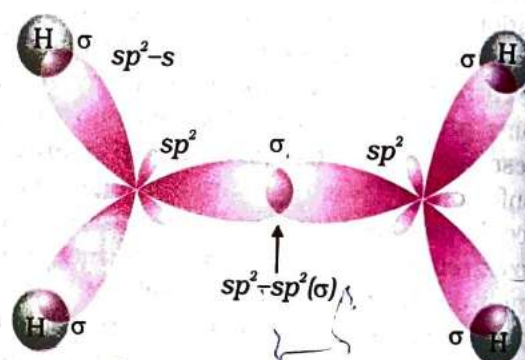
Fig. 13.4 Orbital picture of ethene depicting \sigma bonds only
