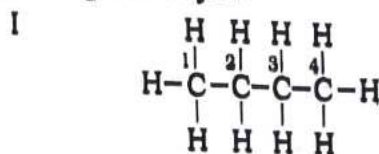
Butane (n-butane), (b.p. 273 K)
