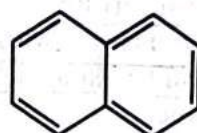
Naphthalene
