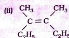
cis -3, 4-Dimethylhex-3-ene
