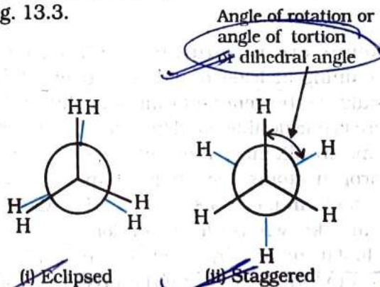
Fig. 13.3 Newman's projections of ethane
