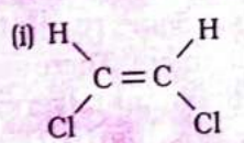
cis -1, 2-Dichloroethene
