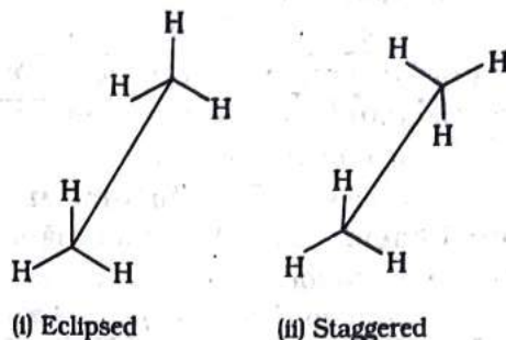
Fig. 13.2 Sawhorse projections of ethane
