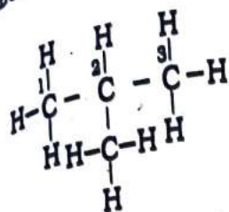
2-Methylpropane (isobutane) (b.p. 261 K)
