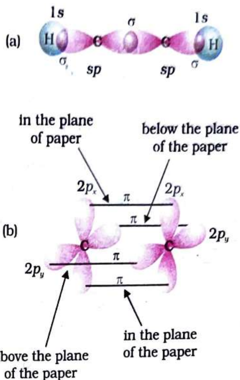
Fig. 13.6 Orbital picture of ethyne showing (a) sigma overlaps (b) pi overlaps.
