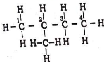
2-Methylbutane (isopentane) (b.p. 301 K)
