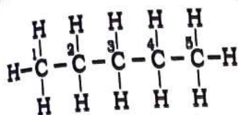
Pentane (n-pentane) (b.p. 309 K)
