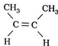
cis-But-2-ene (b.p. 277 K)
