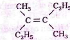
trans -3, 4-Dimethylhex-3-ene
