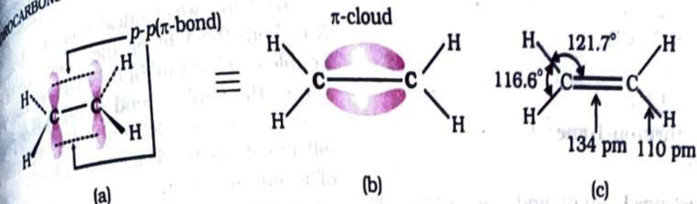
13.5 Orbital picture of ethene showing formation of (a) \pi -bond, (b) \pi -cloud and (c) bond angles and bond lengths
