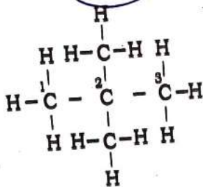
2,2-Dimethylpropane (neopentane) (b.p. 282.5 K)
