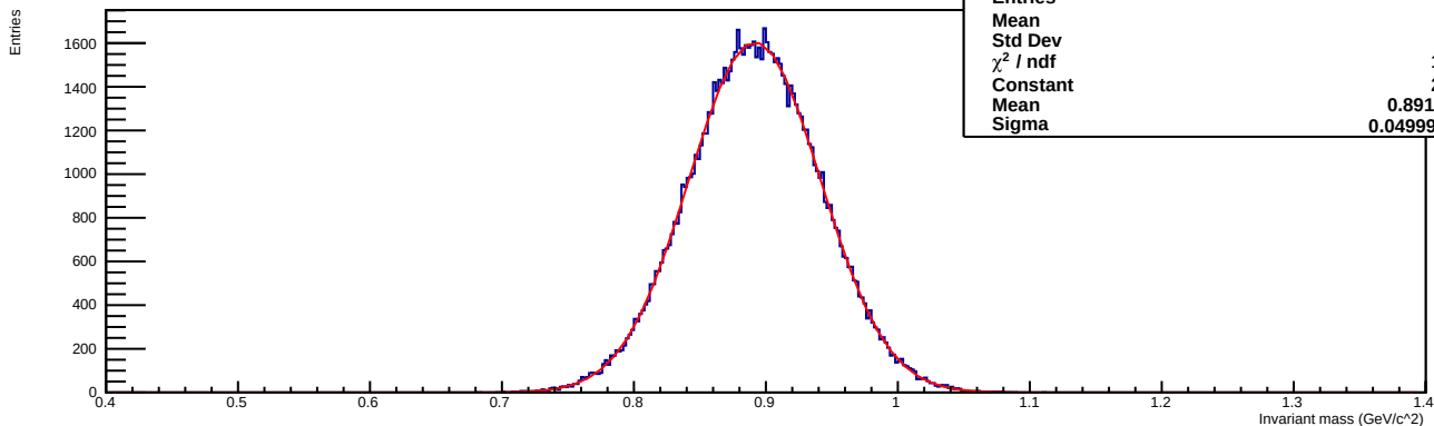
Invariant mass (decay products)
